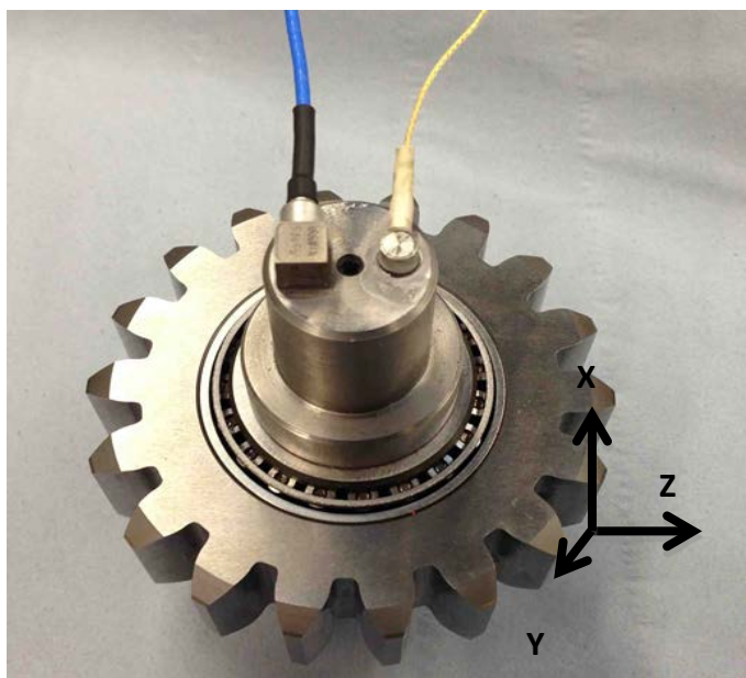
Figure 7 Vibration (left) and AE (right) sensor location
