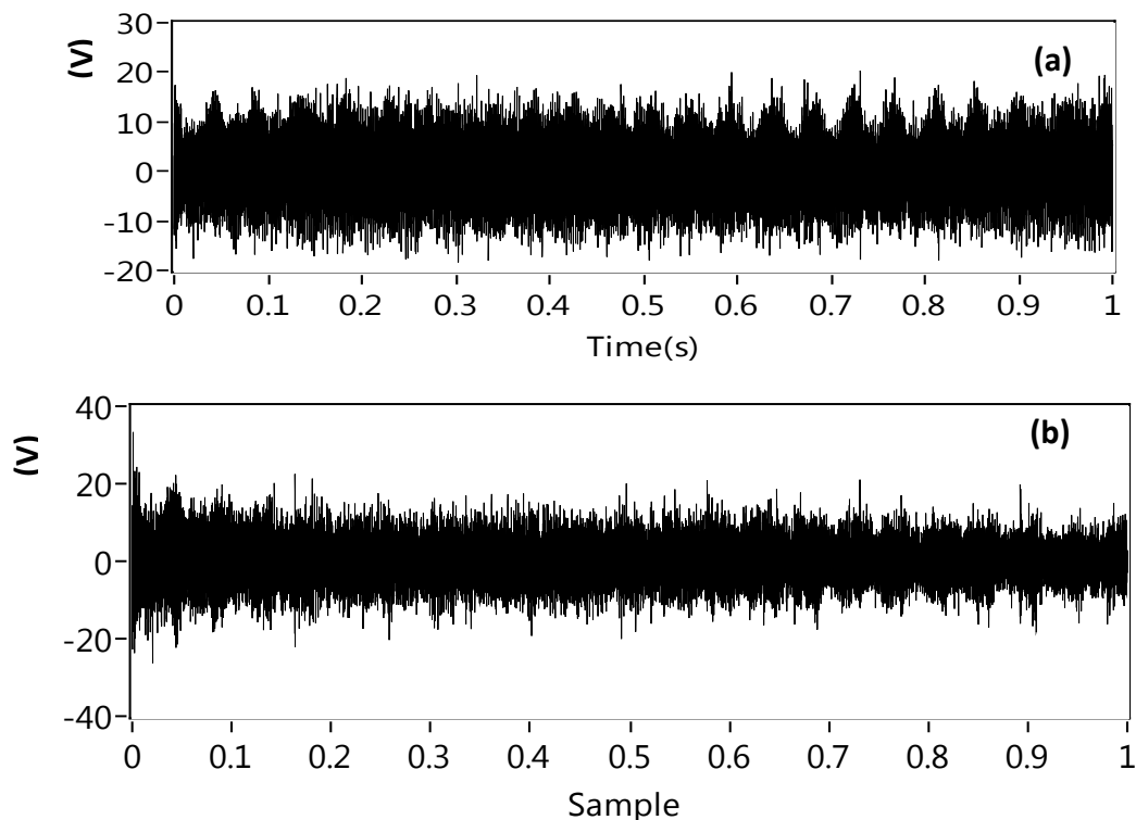
Figure 9 Time waveform of vibration signatures (a) before and (b) after separation for small defect
