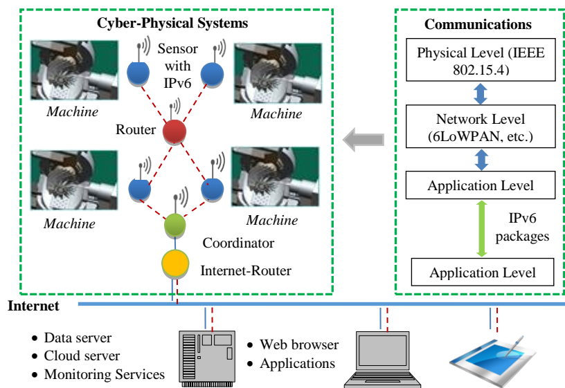
Figure 10: CPS for collecting and monitoring energy Big Data.
