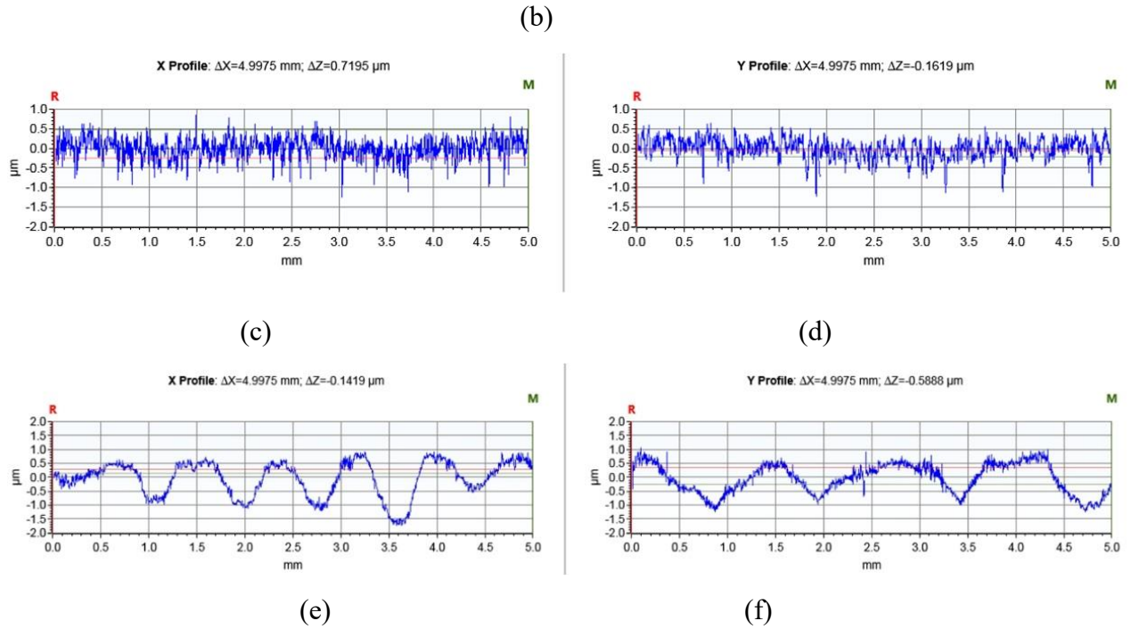
FIGURE 6 A 2-D SURFACE TOPOGRAPHY OF TI-6AL-7NB ALLOY
