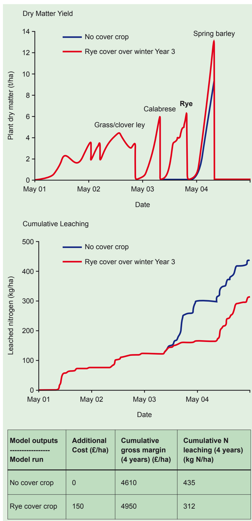
7 Selected outputs (dry matter yield, nitrate leaching and economic performance) from an example simulation of the EU_Rotate-N model
