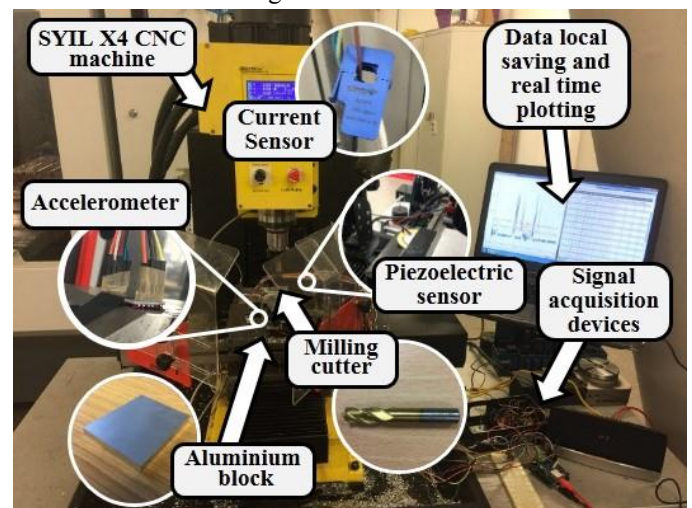
Fig. 2. System setup of machining process monitoring
