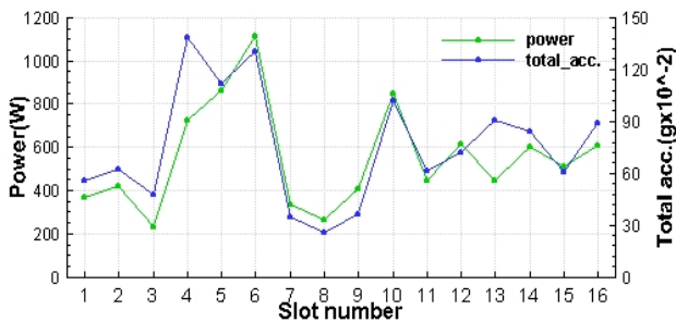
Fig. 8. Power and total acceleration for 16 slots
