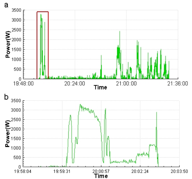
Fig. 4. (a) Power against time; (b) The enlarged failure zone (red box in (a))
