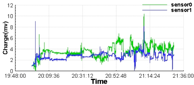
Fig. 7. Charge against time for the piezoelectric sensor
