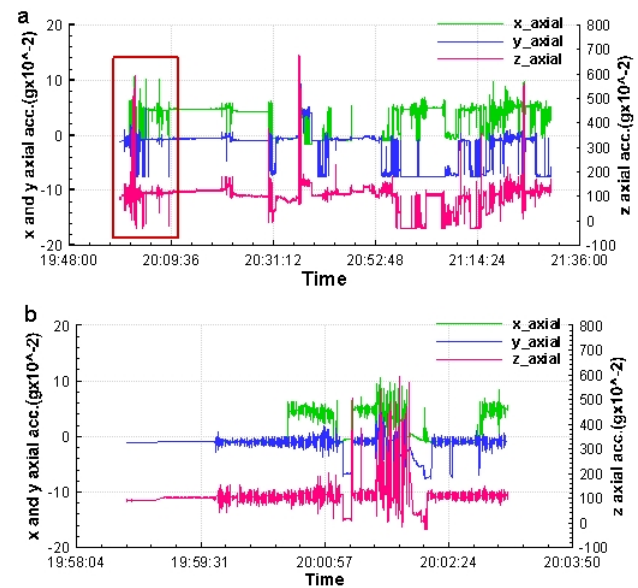
Fig. 5. (a) Acceleration against time; (b) The enlarged failure zone (red box in (a))
