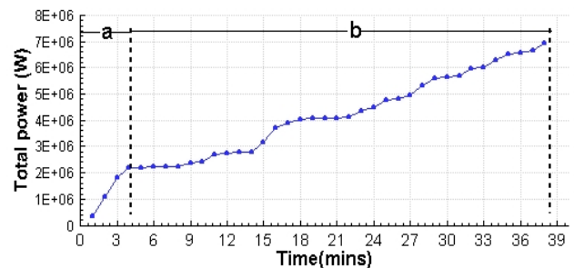
Fig. 10. Power superposition
