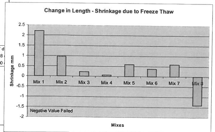
Figure 6. Freeze-Thaw results.
