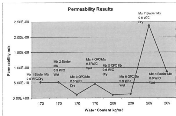
Figure 8. Permeability Results
