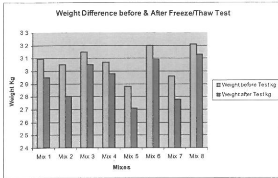
Figure 7. Weight Difference before and after Freeze/Thaw
