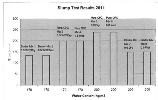
Figure 1. Slump values.
