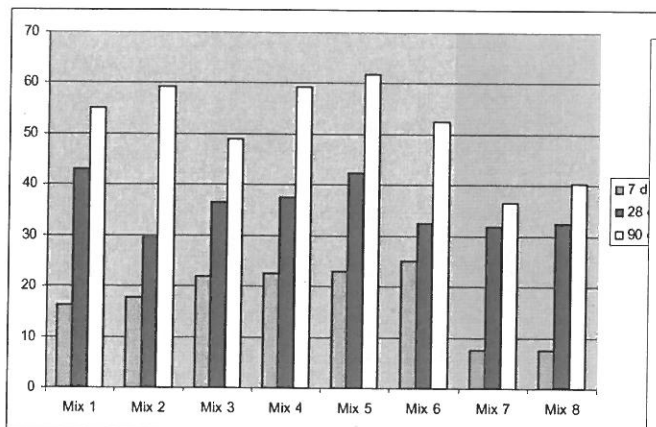
Figure 4. Compressive strength of 100mm cubes
