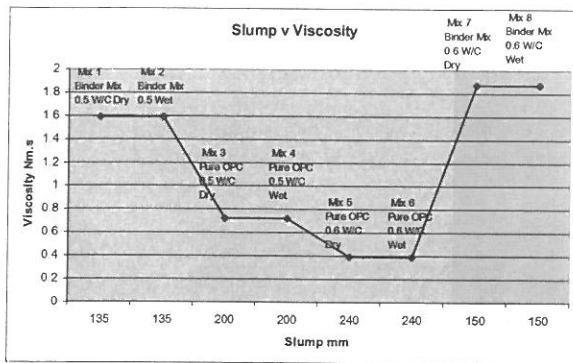
Figure 3. Slump vs viscosity.
