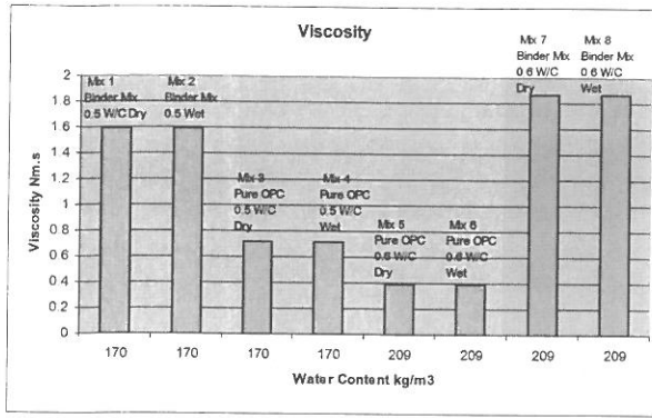
Figure 2. Viscosity results.
