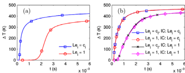
Fig. 1. Temperature rise \Delta T computed using detailed chemistry and different transport models for (a) IML flamelets and (b) ICF flamelets. In fig. (b), different transport models have been used to compute the initial condition (IC) for the ICF flamelets. Case D25H2.
