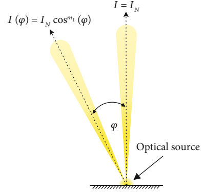
FIGURE 5: Lambert radiator.
