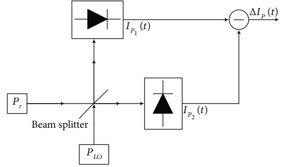
FIGURE 10: Configuration for a balanced PD.
