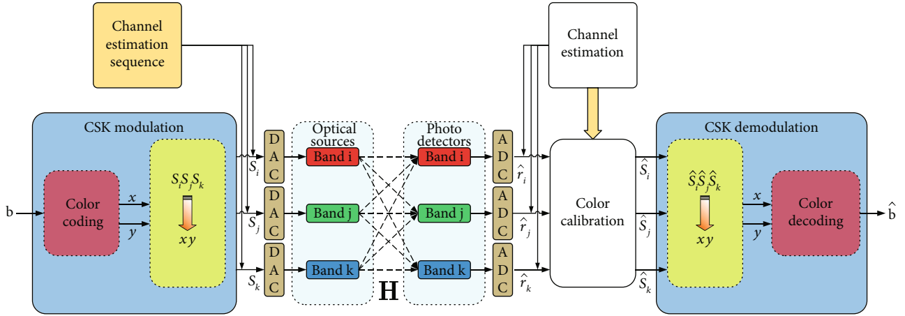
FIGURE 21: M -ary CSK functional system block diagram.
