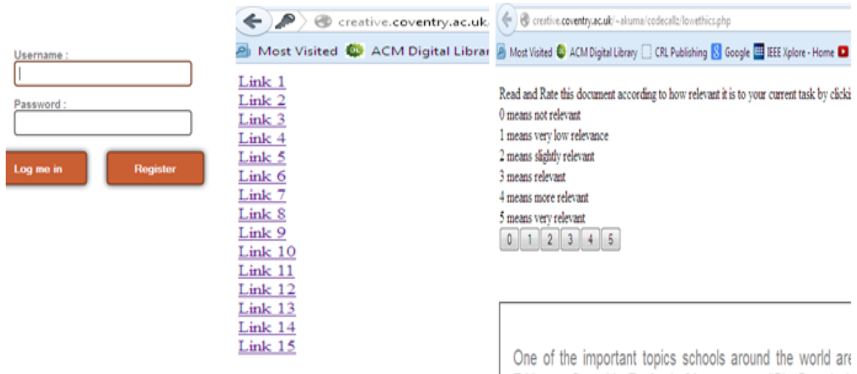
Figure 3.2: Login page, Index page with links to the 15 documents and document page with explicit rating buttons
