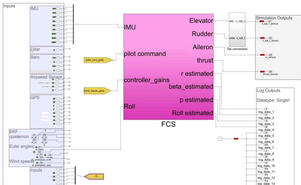
Figure 20. Example Nano Talon flight control model for Simulink/VFTE lateral flight co-simulation (Developed from Alphalink Engineering GmbH (Berlin, Germany) training resources).
