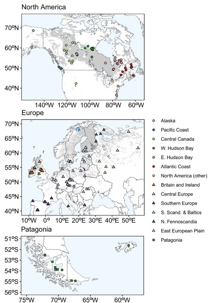
Fig. 1. Site map of peatland record locations and their sub-region. Symbols with a white fill indicate that no charcoal was present throughout a record. Grey shading denotes peatland areas sourced from PEATMAP (Xu et al., 2018).
