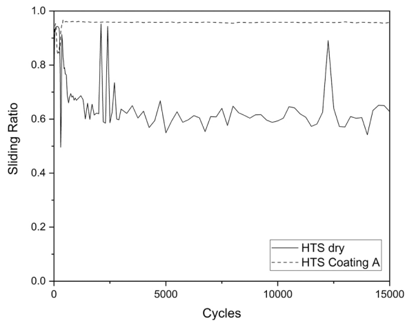
Fig. 3. Sliding ratio variation with cycles for uncoated substrate, and Coating A.
