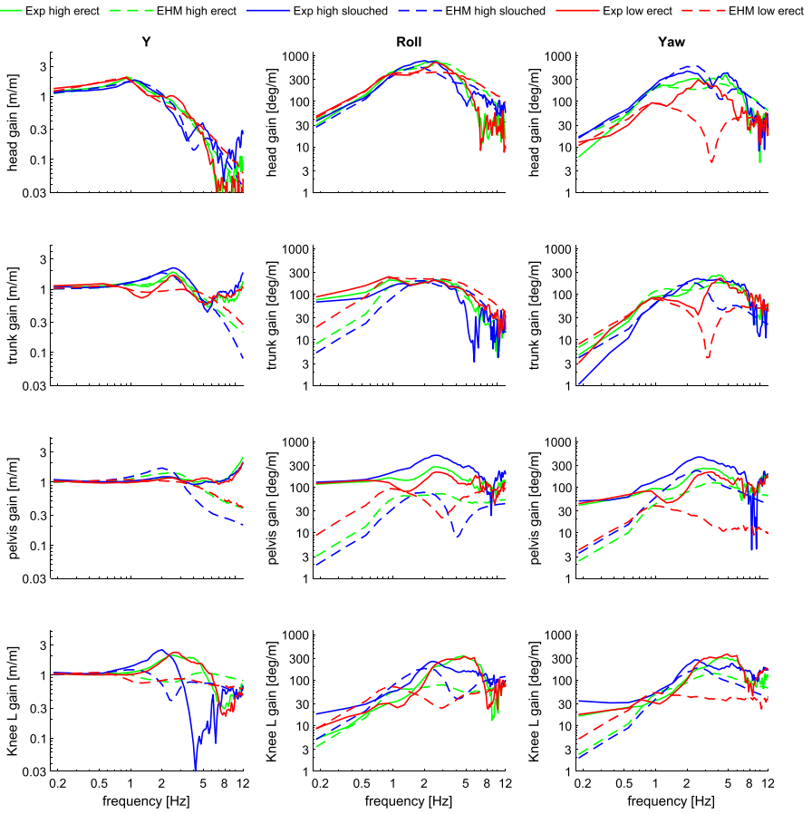
Fig. 19 Experiment vs. EHM model in lateral loading in 3 postures, with MB seat model without contact [Units: translational gain (m/m) and rotational (deg/m)] (Color figure online)
