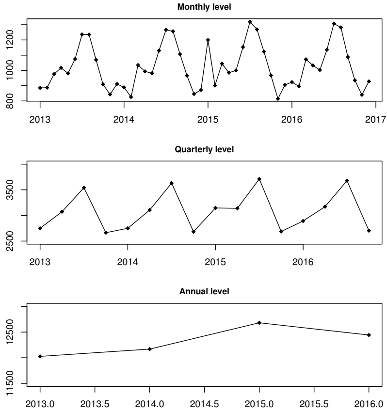
Figure 1: Original time series sampled at a monthly frequency and aggregated at quarterly and annual levels.
