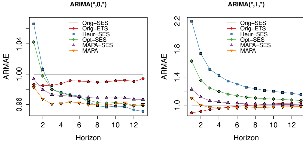
Figure 2: ARMAE per horizon for simulated ARIMA(*,0,*) and ARIMA(*,1,*) .
