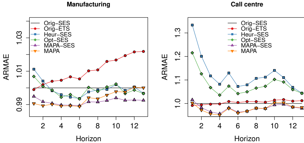
Figure 3: ARMAE per horizon for real datasets.
