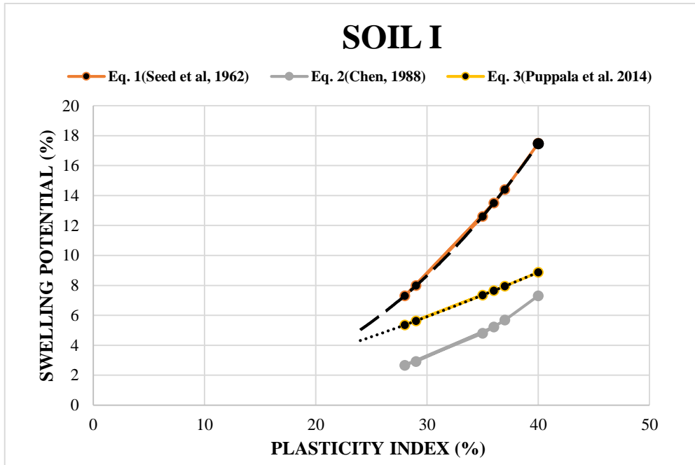
Figure 4a. Relationship between Plasticity Index & Swelling Potential
