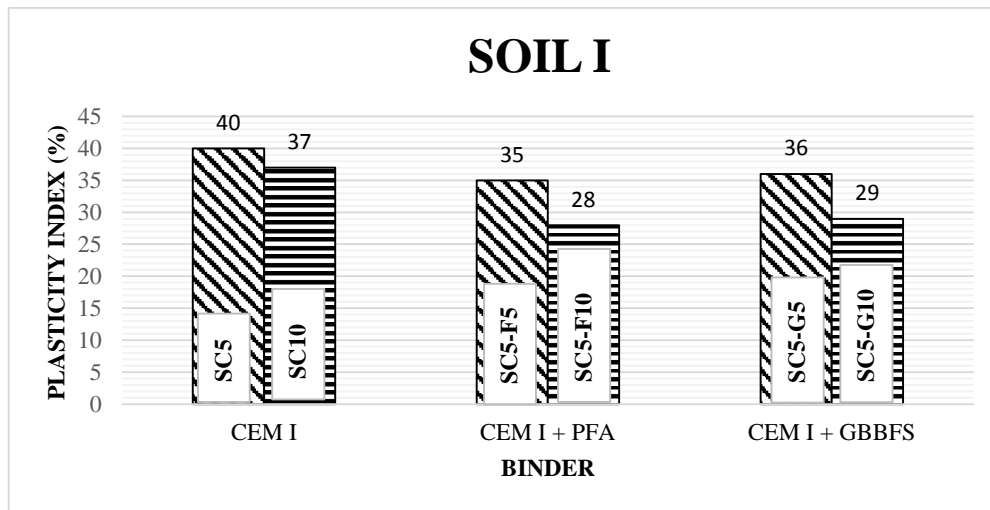
Figure 2a. Variation of Plasticity Index with soil – binder content
