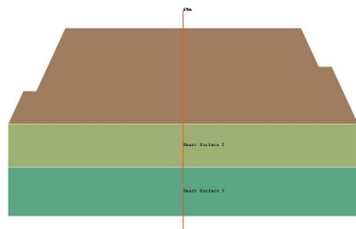
Figure 3. 2D Embankment Model Having Boundary Conditions.
