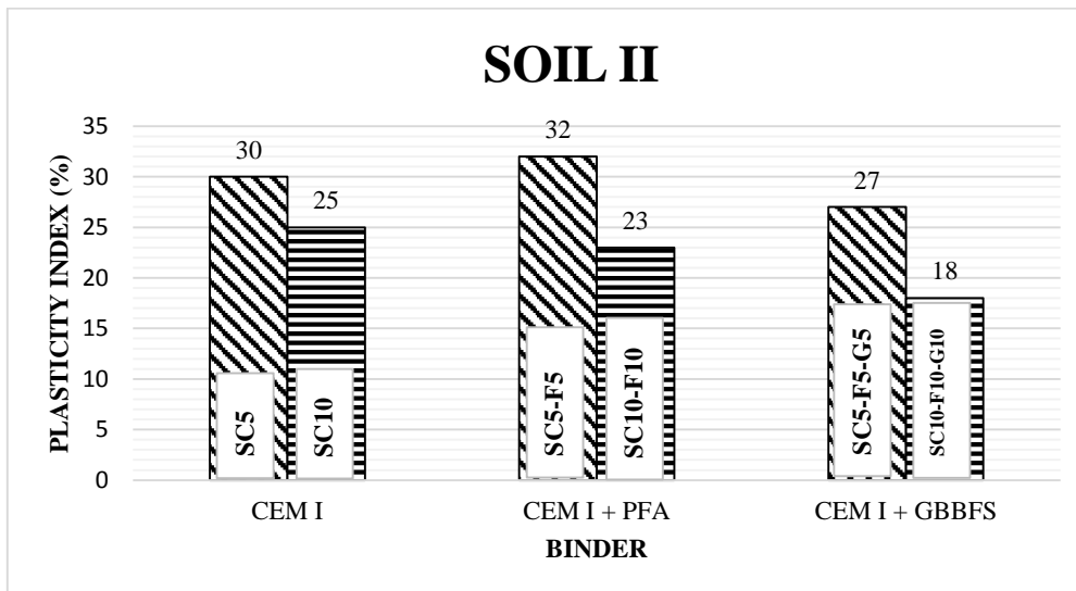
Figure 2b. Variation of Plasticity Index with soil – binder content
