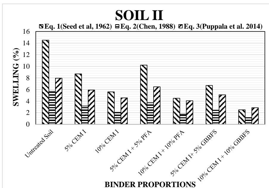
Figure 3b. Variation of Free Swelling with Binder Proportions for Soil II
