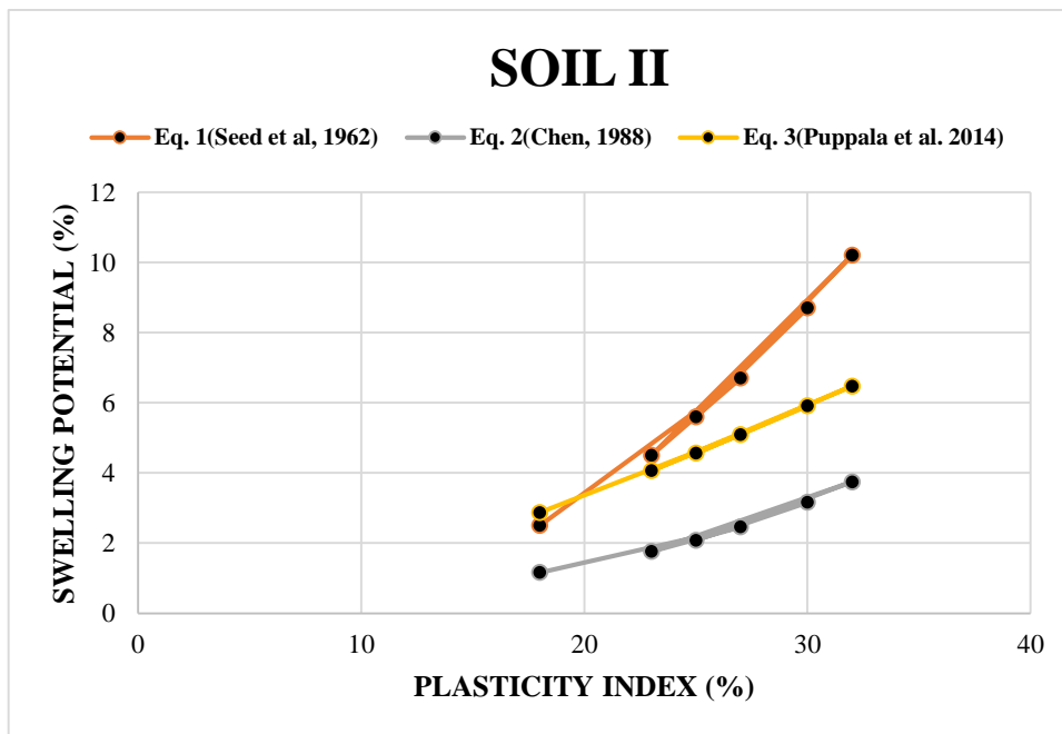
Figure 4b. Relationship between Plasticity Index & Swelling Potential
