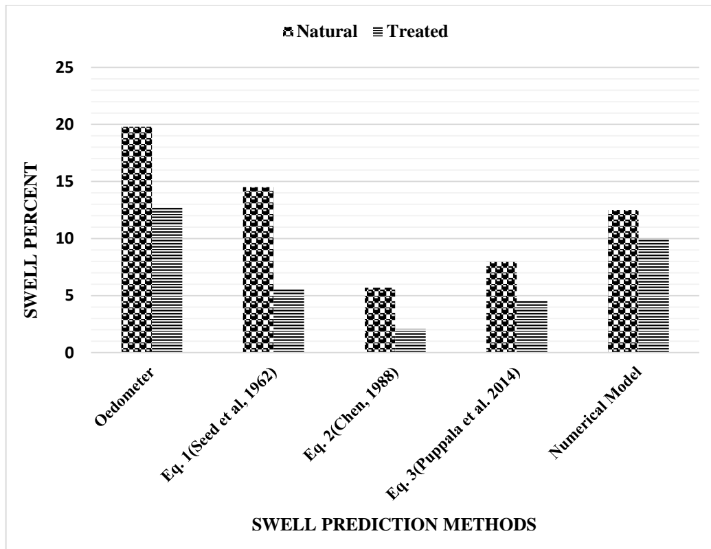
Figure 5. Variation of Swell Prediction Methods
