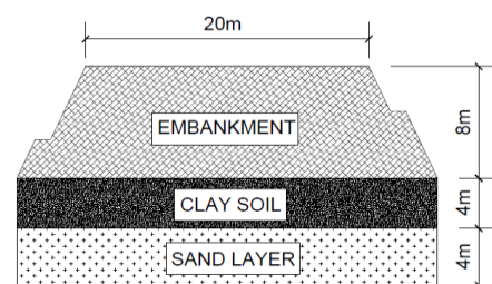
Figure 2. Embankment Setup with Dimensions.
