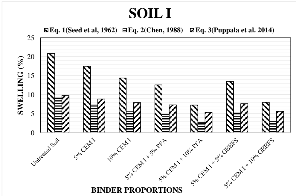
Figure 3a. Variation of Free Swelling with Binder Proportions for Soil I
