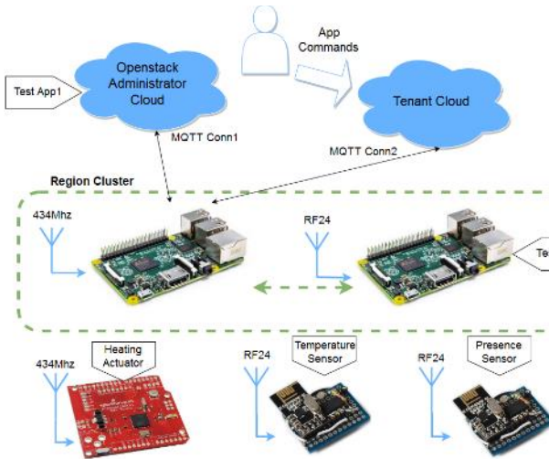
Fig. 4. Distributed Control and Metering Application
