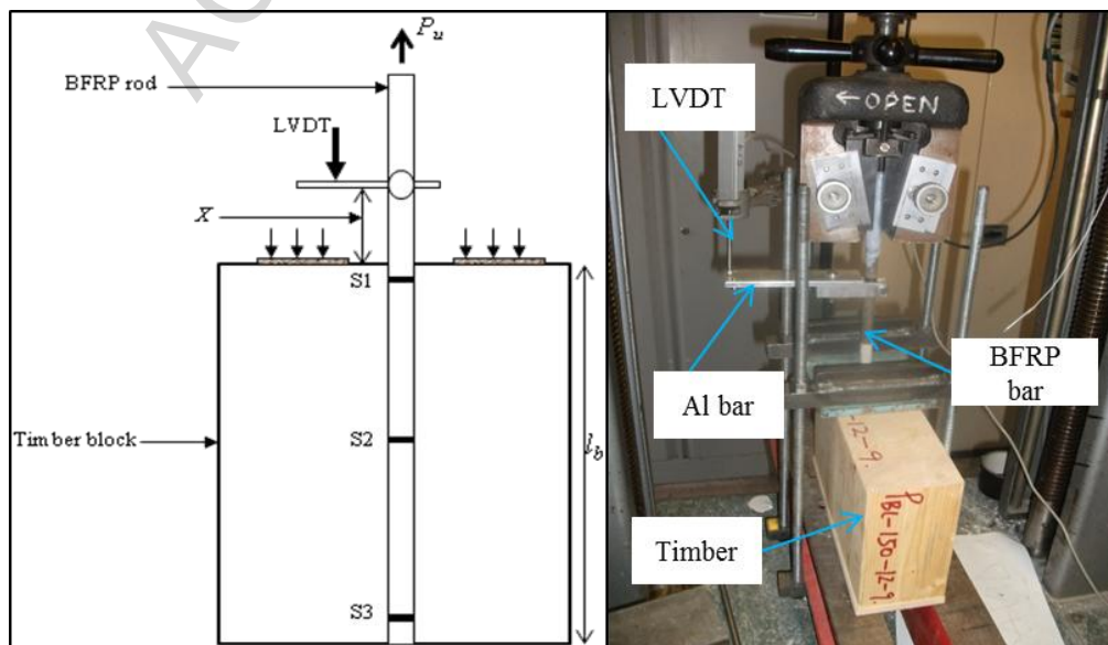
Figure 6: Test set up and instrumentation.
