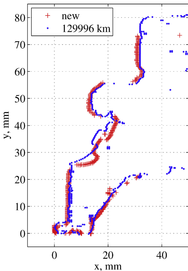
Fig. 11. Comparisons of the main spring geometries: static v. s. creep deformation.
