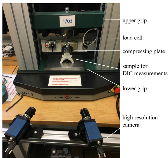
Fig. 2. Static compression test rig with digital image correlation.
