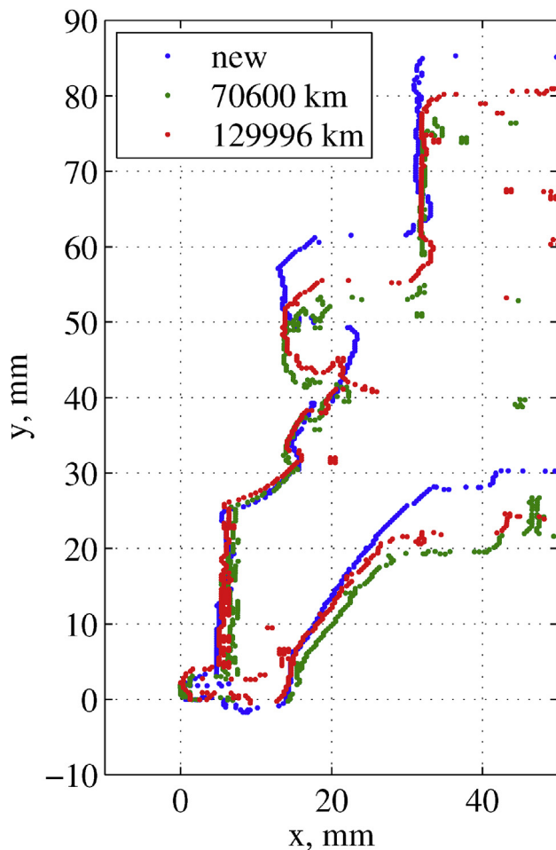
Fig. 7. Comparisons of the main spring geometries for the engine mounts in three different ageing conditions.
