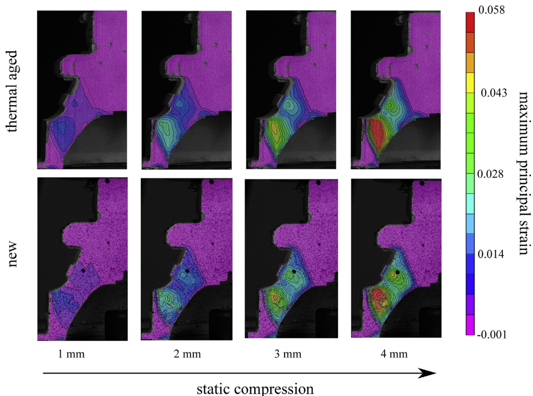
Fig. 5. Maximum principal strain distributions in the main spring for both new and thermally-aged engine mounts when subjected to different amounts of static compressions.
