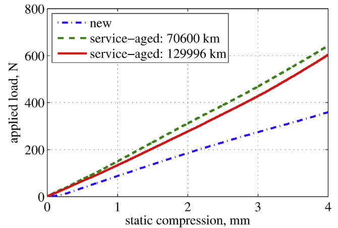
Fig. 6. Load-deflection data for the main springs with different service mileages.
