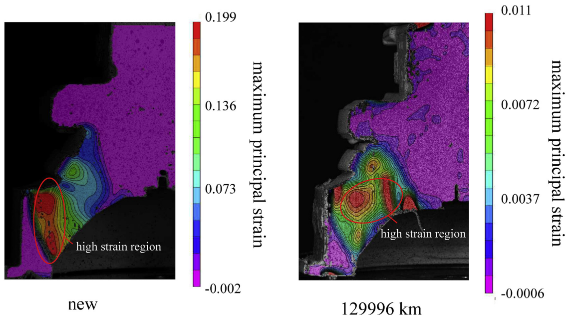
Fig. 10. Maximum principal strain distribution at the same height of 72 mm: (a) Sample 1 (New) under 11 mm of static compression deflection and (b) Sample 3 (service-aged with mileage of 129,996 km) under 1 mm of static compression deflection.
