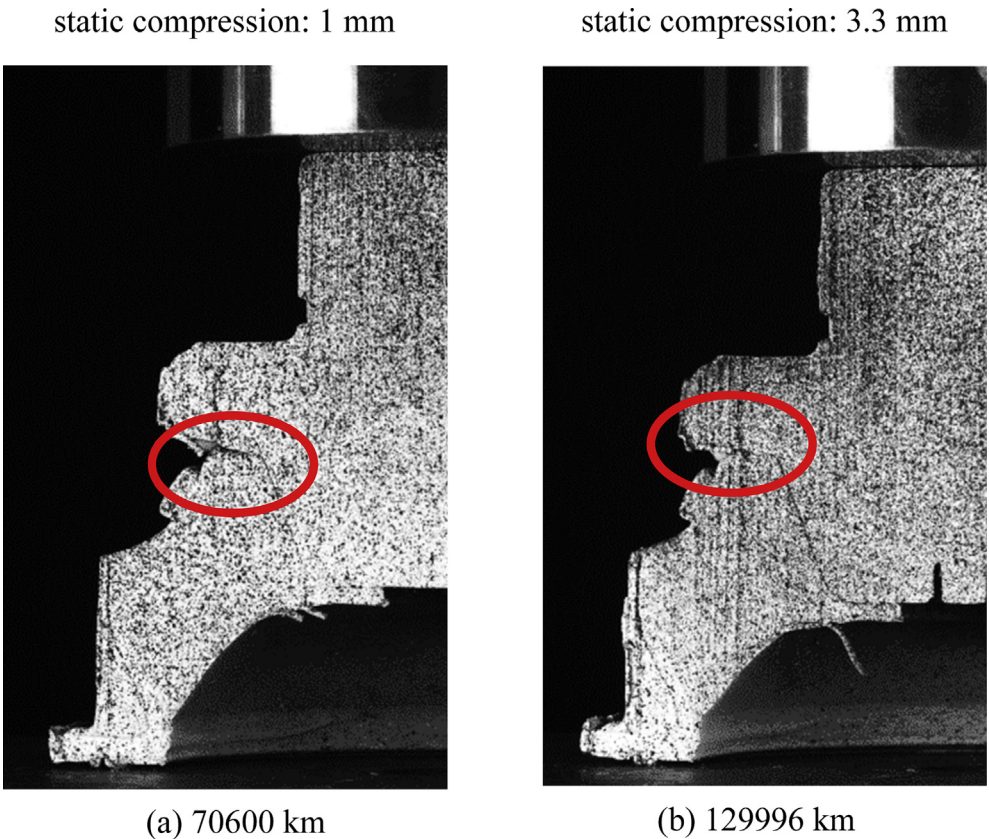
Fig. 9. Development of contact regions for service-aged engine mounts.
