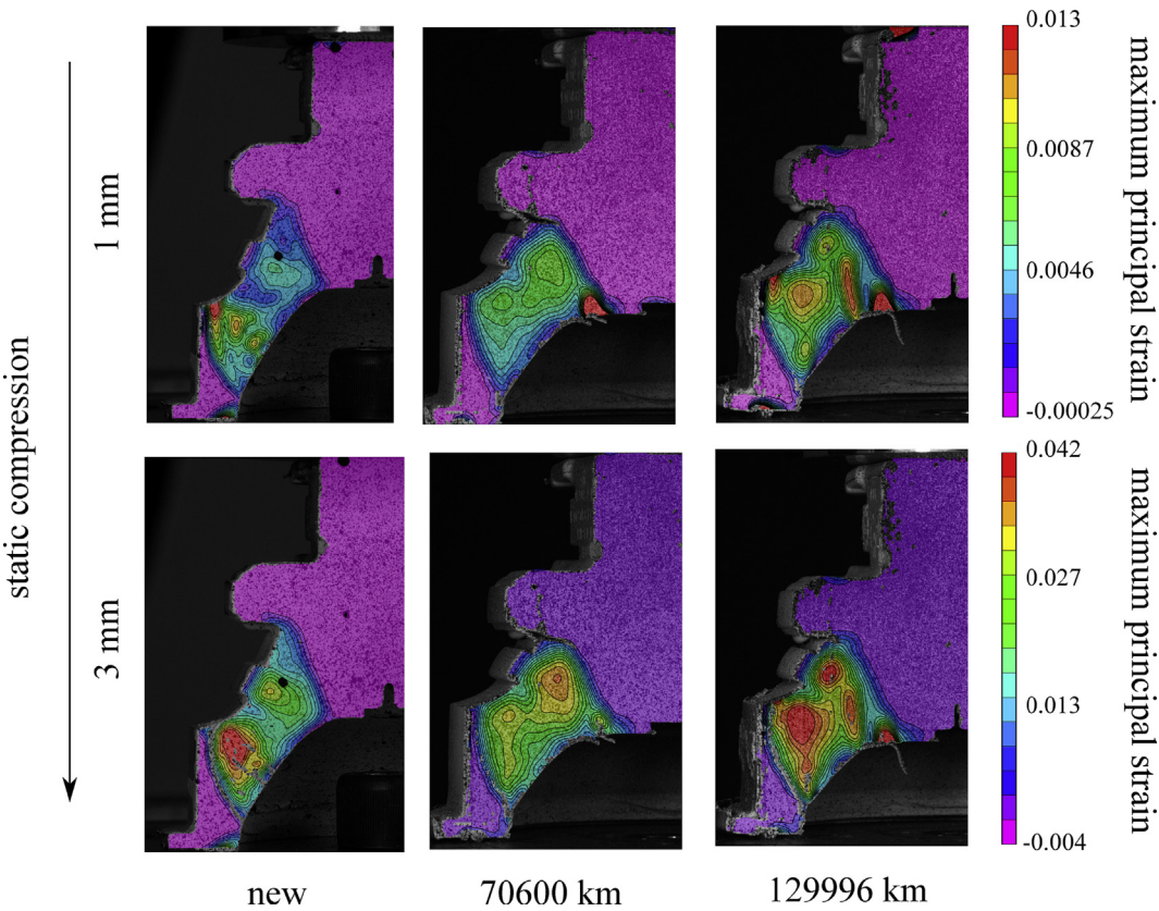
Fig. 8. Cross-sectional maximum principal strain distribution for main springs at different ageing conditions.
