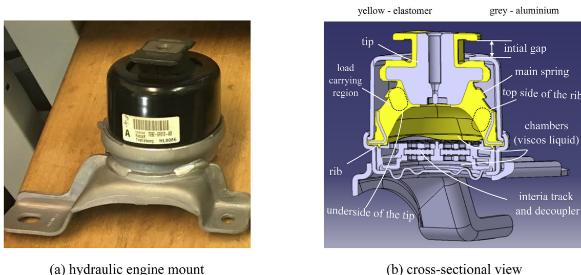
Fig. 1. Hydraulic engine mount and its components.
