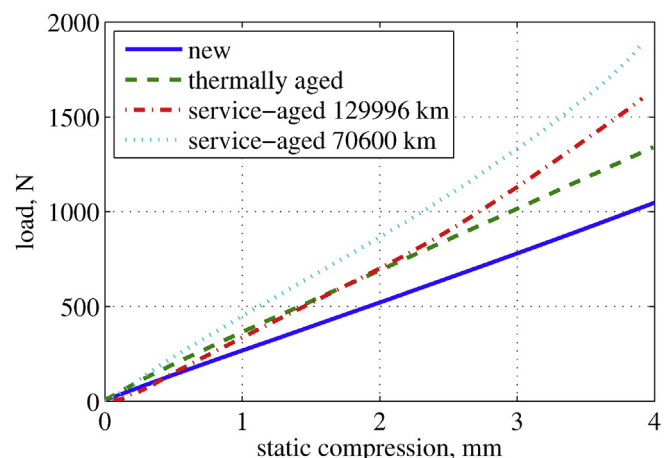
Fig. 4. Load-deflection data for the selected engine mounts.
