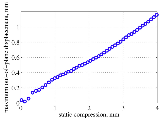
Fig. 3. Typical maximum out-of-plane displacements for a service-aged engine mount.
