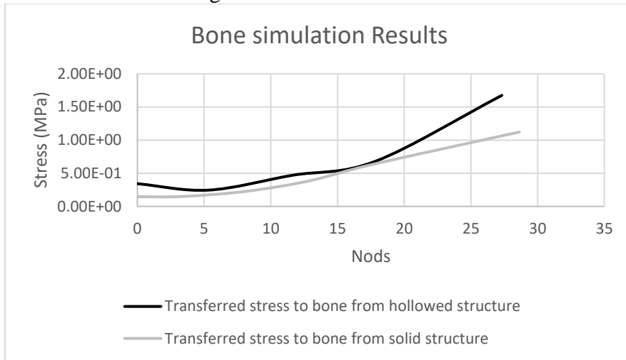
Figure 3: Transferred Stress to bone from two specimens
