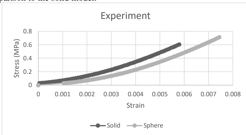
Figure 4: Stress-strain graph of solid and hollowed spheres closed to the surface structure
