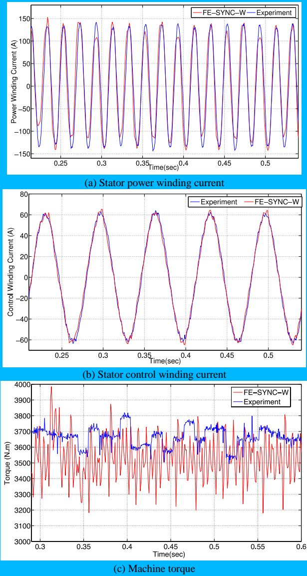
Fig. 3. Comparison of stator currents and machine torque obtained from experimental tests and non-linear FE analysis.
