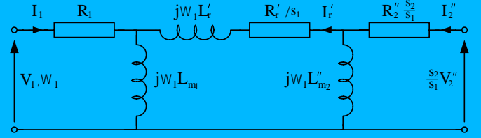
Fig. 2. Simplified equivalent circuit of the BDFM [10]
