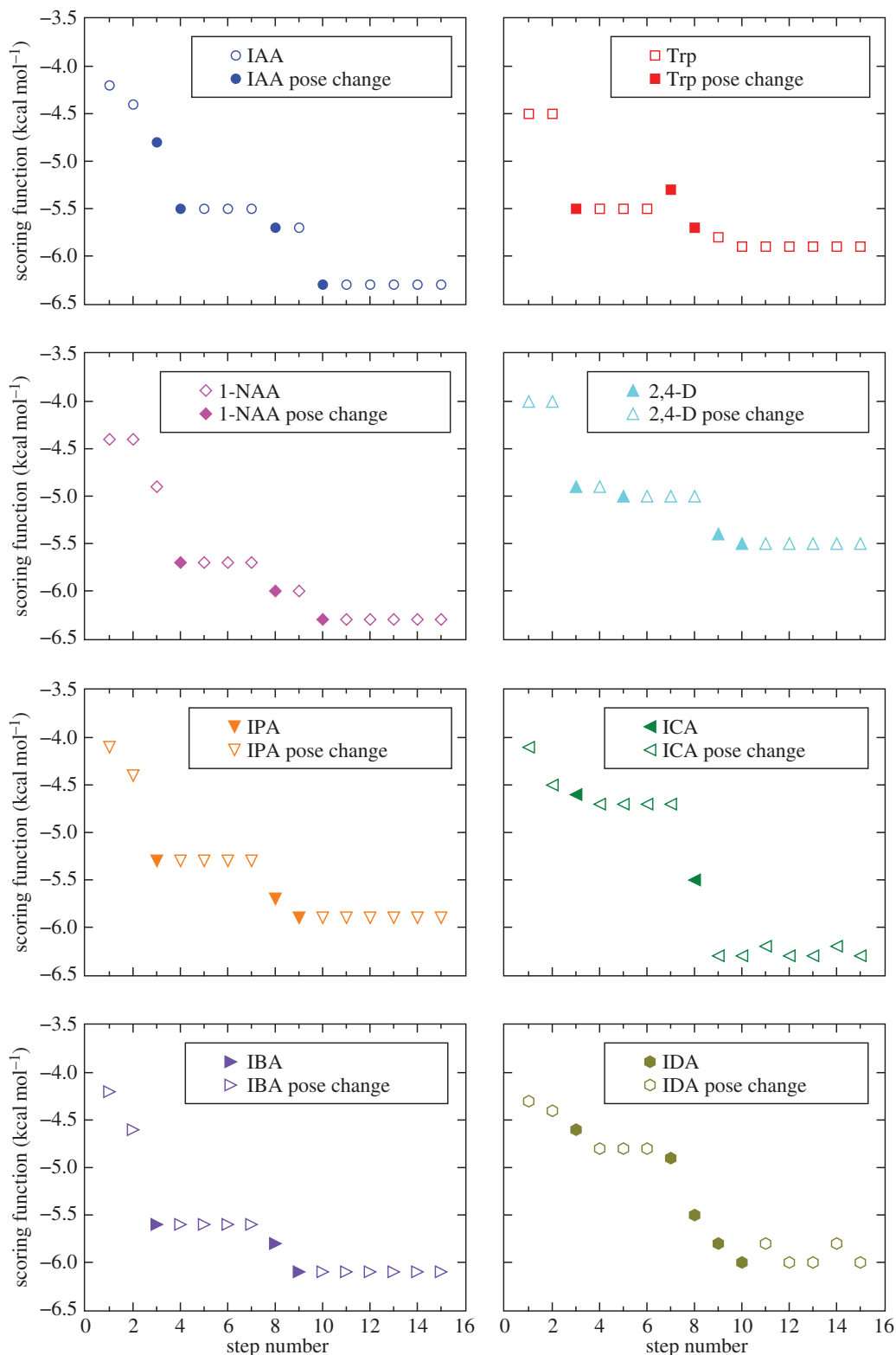
Figure 3. Best scores of docked poses along the transect for all compounds tested, namely IAA (blue circles), Trp (red squares), 1-NAA (magenta diamonds), 2,4-D (cyan triangles), IPA (orange triangles), ICA (green triangles), IBA (violet triangles) and IDA (olive hexagons). Each step represents the progression of the search space by 1 Å in the direction of the pocket bottom. Filled symbols indicate steps at which a significant change in depth or orientation of the docked pose occurs.
