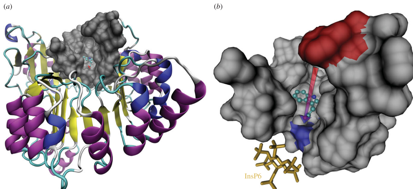
Figure 1. The deep binding pocket on TIR1. The binding site of TIR1 is not a shallow surface indentation but a deep pocket, shown in SURF representation in panel (a) superimposed on the cartoon of the whole receptor (2P1P). The residues comprising the binding pocket, isolated and shown from a closer point in panel (b), are contributed by seven non-sequential leucine-rich repeats [1]. The two reference residues Phe-351, in red, and Arg-403, in blue, indicate the mouth and the bottom of the pocket, respectively. Their distance, indicated by the arrow in the figure and corresponding to the pocket depth, is 16.5 Å. IAA is shown in CPK representation, and InsP6 is on the bottom left in bond representation. All three-dimensional molecular visualizations were produced using VMD [19,20].
