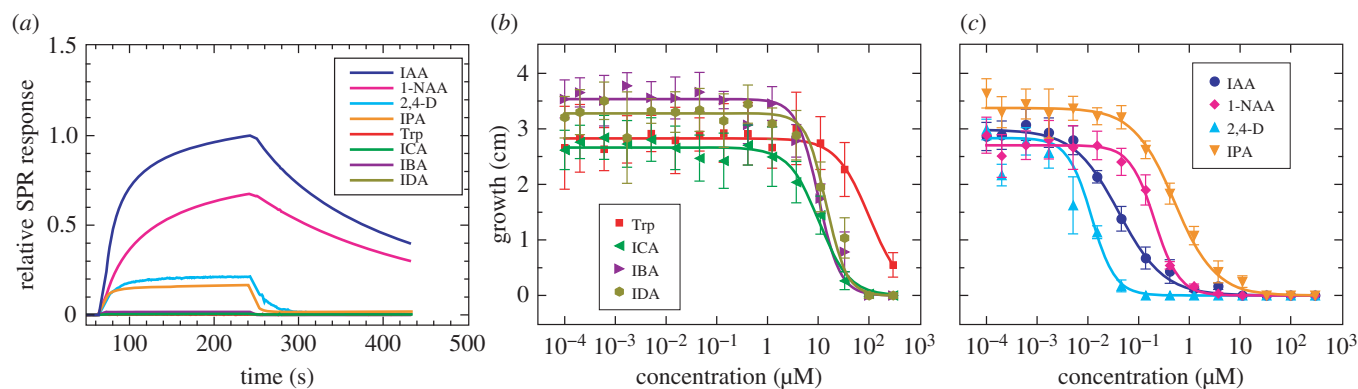
Figure 7. Surface plasmon resonance and root-growth assay results confirm the numerical predictions. (a) The results from SPR experiments show that Trp (red line), ICA (green line), IBA (violet line) and IDA (olive line) do not bind TIR1 at all. Conversely, 1-NAA (magenta line), 2,4-D (cyan line) and IPA (orange line) all bind, although with differing activities from IAA (blue line). All compounds were tested at 50 μM. (b,c) Root-growth inhibition measurements substantially confirm these results, revealing that Trp (red squares), ICA (green triangles), IBA (violet triangles) and IDA (olive hexagons) do not inhibit root growth up to extreme concentrations. In (c), 1-NAA (magenta diamonds), 2,4-D (cyan triangles) and IPA (orange triangles) are all active auxins. Derived IC 50 values are given in table 1.
