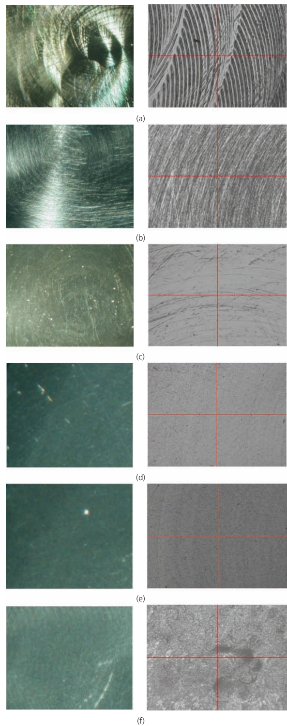
Figure 6. Microscopic view of the finished surfaces: (a) FM sample; (b) SP-polished sample; (c) DP-polished sample; (d) AF-coated sample; (e) Triton-coated sample; and (f) titanium dioxide-coated sample
