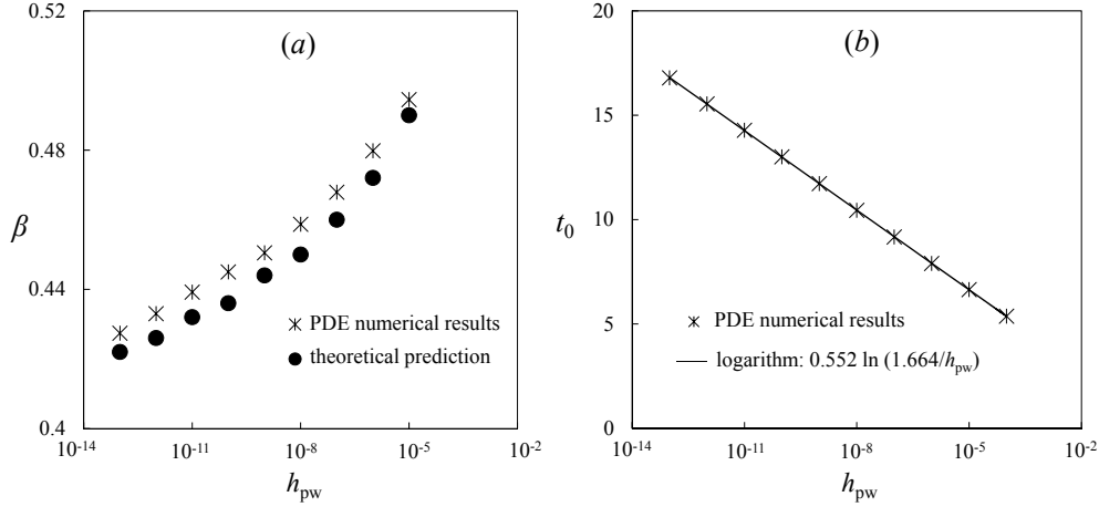
FIGURE 12. Influence of the thickness of the prewetting film h_{pw} on (a) the scaling exponent \beta and (b) the healing time t_0 . (a) A thinner prewetting film corresponds to a smaller value of scaling exponent \beta , which is also consistent with the theoretical calculations as described in § 2.3.3. (b) A thinner prewetting film corresponds to a greater healing time t_0 , and the numerical data suggests a logarithmic fit for the dependence of t_0 on h_{pw} .
