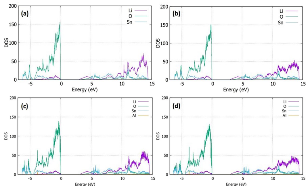
Figure 7. The PDOS calculated using DFT for the (a) \text{Li}_2\text{SnO}_3 perfect cell (b) \text{Li}_2\text{SnO}_3 with Li interstitial (c) Al – Doped \text{Li}_2\text{SnO}_3 and (d) Al- Doped \text{Li}_2\text{SnO}_3 with Li interstitial.
