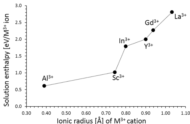
Figure 5. Enthalpy of solution of R_2O_3 ( R = \text{Al}, \text{Sc}, \text{In}, \text{Y}, \text{Gd} and \text{La} ) with respect to the R^{3+} ionic radius in \text{Li}_2\text{SnO}_3 .
