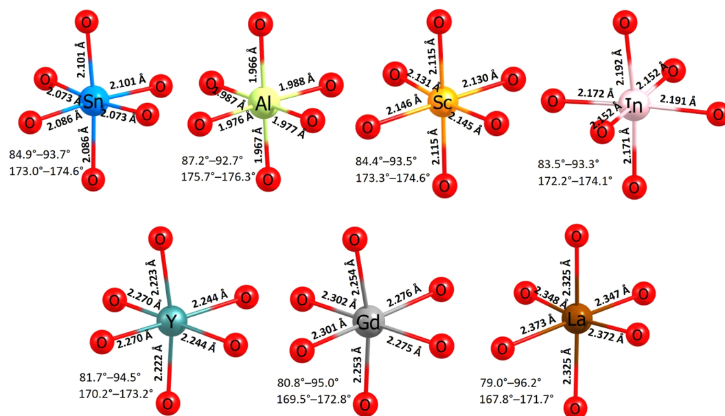
Figure 6. Octahedral \text{SnO}_6 unit in the relaxed structure of undoped \text{Li}_2\text{SnO}_3 and the coordination formed by the dopants on the Sn site with neighbor oxygen.
