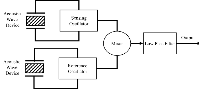
Figure 10. Frequency Measurement configurations of acoustic wave devices for particle sensing: block diagram of a dual configuration with mixing circuitry.
