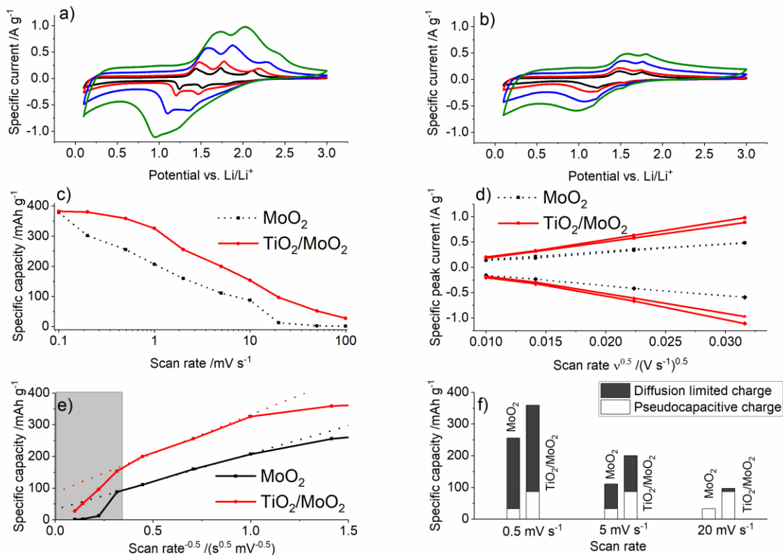
Figure 4. Cyclic voltammograms for a) \text{TiO}_2/\text{MoO}_2 composite and b) \text{MoO}_2 at 0.1, 0.2, 0.5 and 1.0 \text{mV s}^{-1} in black, red, blue and green, respectively. c) Plots of specific capacities over scan rate for both. d) The relationship between specific peak currents and scan rate. e) Plots of specific capacity vs. the reciprocal of the square root of the scan rate (with high scan rate region in grey excluded from analysis) and f) proportion of pseudocapacitive charge storage for both the composite and pure \text{MoO}_2 at scan rates of 0.5, 5 and 20 \text{mV s}^{-1} .
