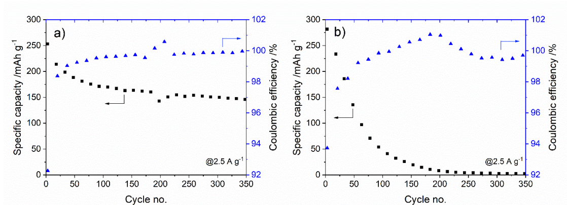
Figure 6. Specific capacities (black squares) and Coulombic efficiencies (blue triangles) for Li-ion half-cells of electrodes made from a) nanocomposite TiO 2 /MoO 2 and b) pure MoO 2 nanoparticles; both at a constant specific current of 2.5 A g -1 .
