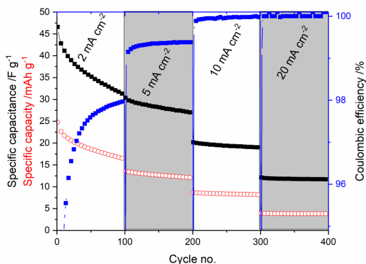
Figure 10. Cyclic charge/discharge measurements of \text{TiO}_2/\text{MoO}_2//\text{AC} Li-ion hybrid electrochemical capacitor at varying current densities.
