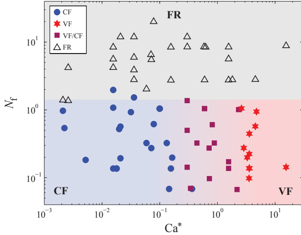
FIG. 4. Phase diagram of drainage in granular media, showing three invasion regimes: viscous fingering (VF), capillary fingering (CF), and fracturing (FR). The tendency to fracture is characterized by the “fracturing number” N_f : drainage is dominated by fracturing in systems with N_f \gg 1 . At lower N_f values, the type of fingering depends on the modified capillary number, Ca^* .
