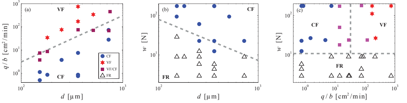
FIG. 3. Phase diagrams of fluid-fluid displacement patterns in the experiments. The diagrams demonstrate how changing the control parameters affects the patterns. Diagram (a) shows that the transition from viscous fingering (VF) to capillary fingering (CF) occurs at q/b \sim d^2 (fixing w=181 N). Intermediate patterns are marked as VF/CF. Diagram (b) shows that the transition from capillary fingering to fracturing (FR) occurs at w \sim d^{-1} ( q=0.1 mL/min). Diagram (c) shows that the transition from fingering to fracturing is independent of q/b ( d=360 μm).
