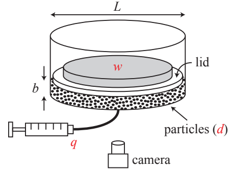
FIG. 1. Experimental setup: a thin bed (thickness b ) of water-saturated glass beads (mean diameter d ) is confined in a cylindrical acrylic cell (internal diameter L ). Vertical confinement is supplied by a weight, w , placed on a disk (“lid”) that rests on top of the beads. The disk is slightly smaller than the cell to allow fluids (but not particles) to leave the cell. Air is injected into the center of the cell at a fixed flow rate q . Time-lapse images are captured by a camera placed underneath the cell.
