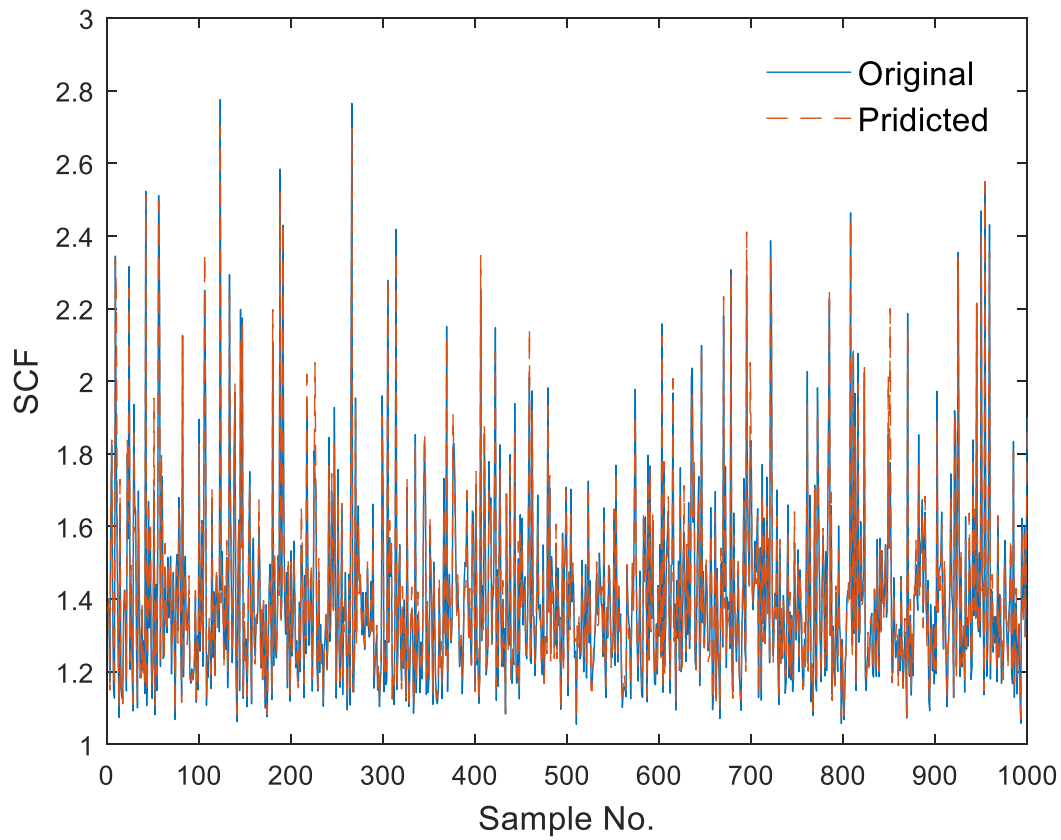
Figure 18. Comparison of original and predicted data
