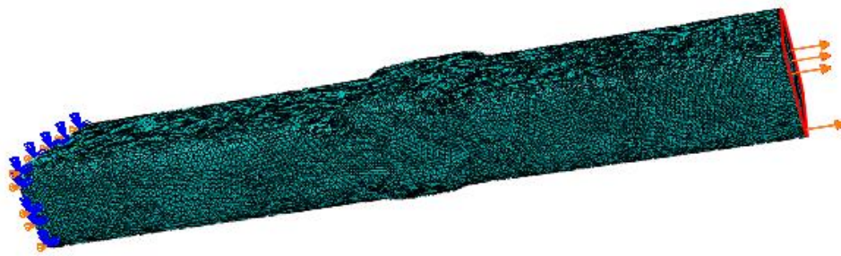
Figure 6. Boundary conditions
