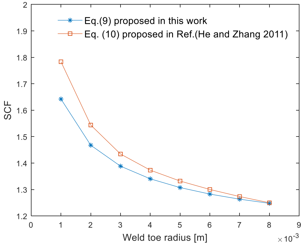
Figure 19. Calculated SCF
