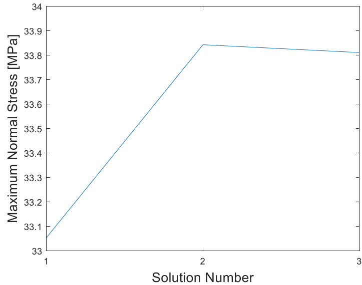
Figure 9. Mesh convergence
