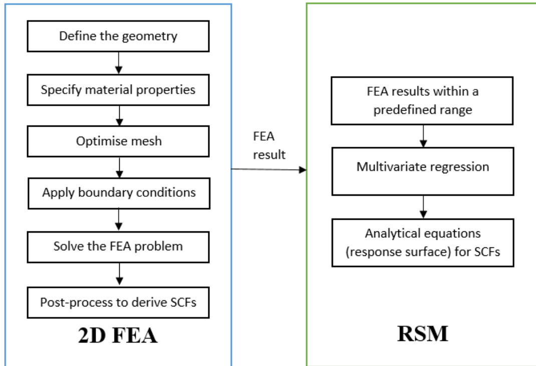
Figure 11. Flowchart of RSM-FEA2D model for calculating SCFs
