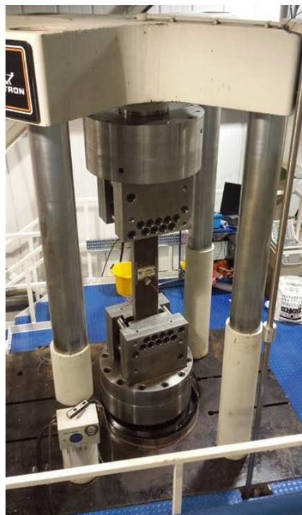
Figure 12. Experimental configuration of large scale dog-bone tests
