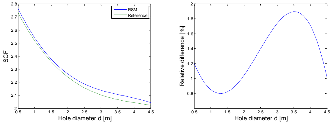
Figure 16. Calculated SCF: a Comparison of SCF obtained from RSM and Reference; b Relative difference
