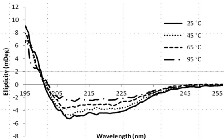
Figure 4 The effect of temperature on A_{2a}R structure revealed by CD spectra of purified A_{2a}R -SMALP
