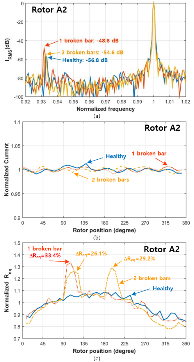
Fig. 14 Comparative test results for the case where 2 broken bars 90 electrical degrees apart cancel out asymmetry (rotor A2): (a) MCSA; (b) single phase rotation test; and (c) normalized R_{eq} measurements of proposed test
