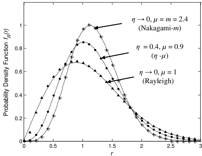
Fig. 1. PDFs of \eta - \mu / inverse gamma composite fading model (continuous lines) for special cases: \eta - \mu (circles), Nakagami- m (asterisks) and Rayleigh (triangles) PDFs.
