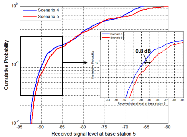
Fig. 10 CDFs for base stations 5 (target base station) during scenarios 4 and 5.
