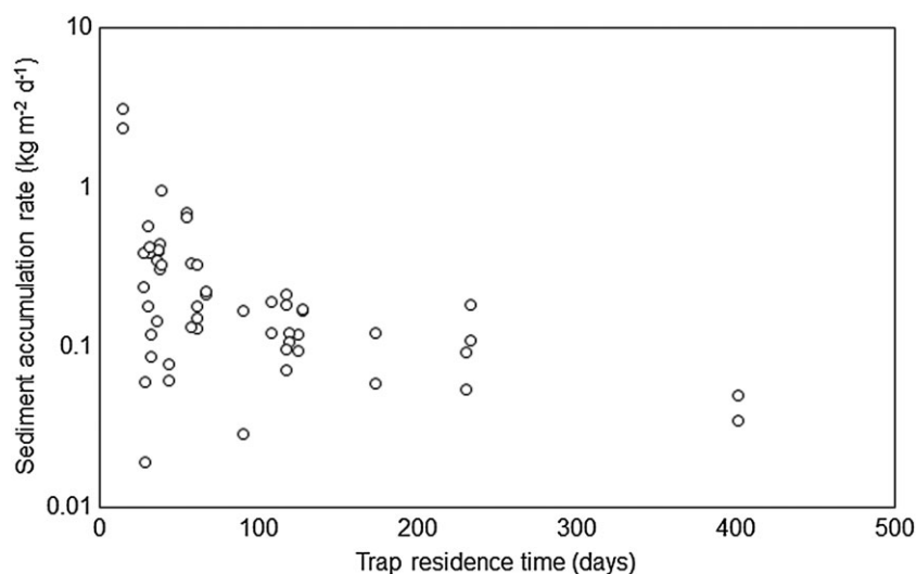
FIGURE 6 Rate of fine sediment accumulation ( \text{kg}/\text{m}^2/\text{day} ) as a function of trap residence time
