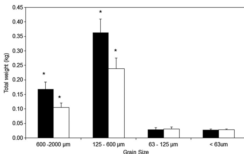
FIGURE 5 Average mass of fine sediment (+1 SE) for grains 600–2,000, 125–600, 63–125, and <63 µm by trap design for all traps installed on the River Tame. Black = vertically extending sediment traps and white = fixed-area sediment traps
