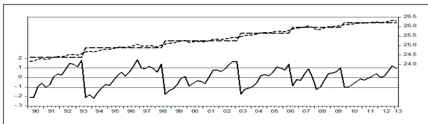
Figure 1: Structural Breakpoints in Malaysian GDP (1990-2014)
