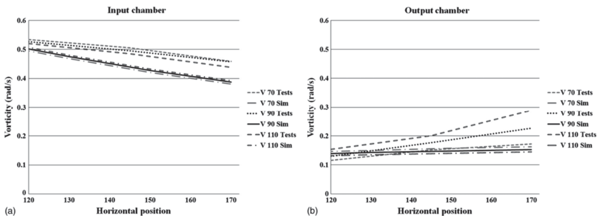
Figure 5. A comparison of vorticity results between the laboratory test and numerical simulation for: (a) the input chamber; (b) the output chamber.
