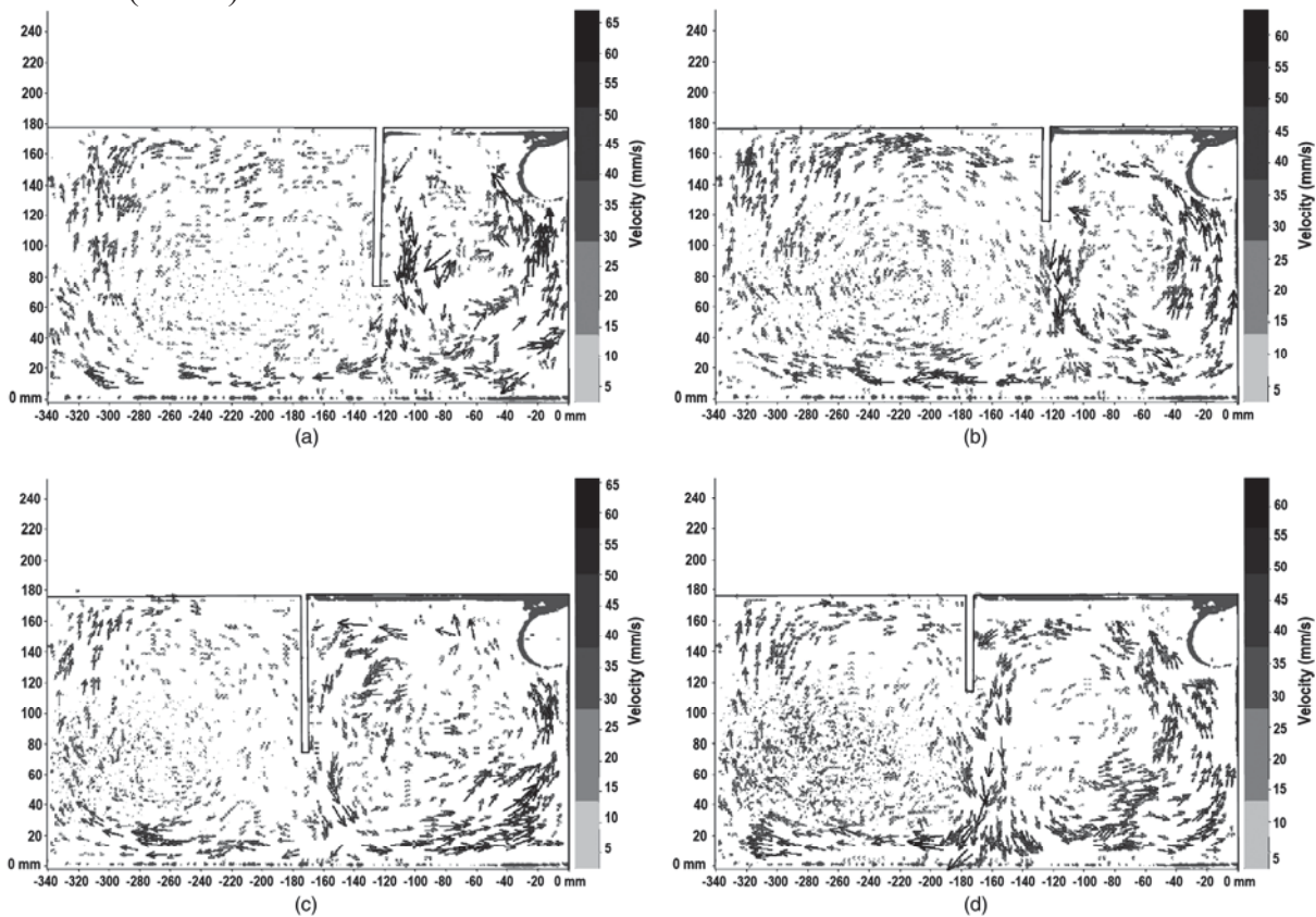
Figure 2. Screen captures in the PIV tests for different flat panel positions: a) H2 – V2; b) H2 – V3; c) H3 – V2; d) H3 – V3.
