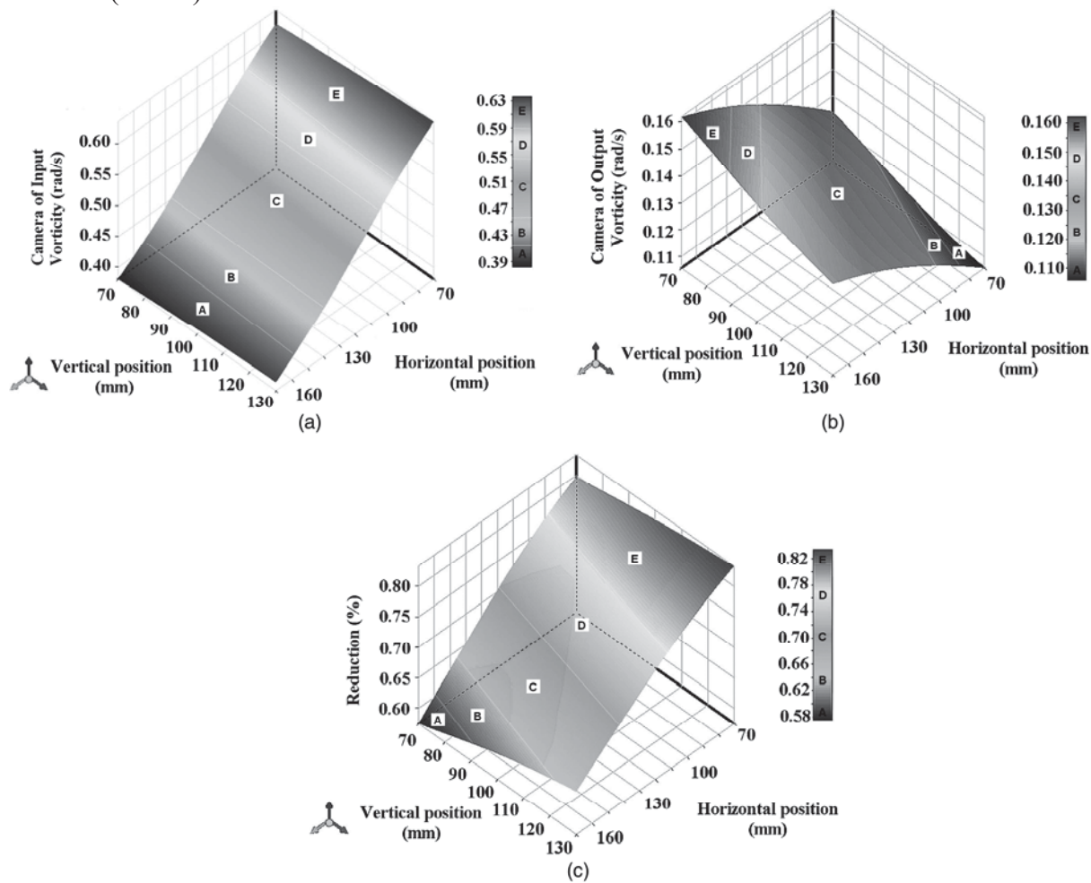
Figure 4. Response surface of the central panel position influence: a) average vorticity in the input chamber; b) average vorticity in the output chamber; c) vorticity reduction.
