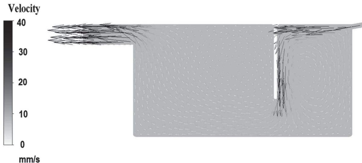
Figure 3. Numerical simulation results: velocity vectors map in the SCPT for a flat panel position of H = 120 mm. and V = 90 mm.
