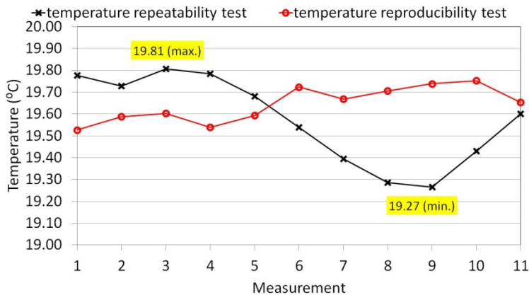
Fig. 4. Laboratory temperature histories during measurements, for repeatability and reproducibility test. Temperature range ( \Delta T ) for repeatability and reproducibility tests were 0.54°C and 0.22°C respectively.
