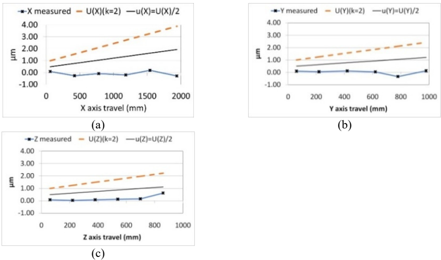
Fig. 3. Axes deviation from zero and axis error as a function of axis travel; (a) X-axis, (b) Y-axis and (c) Z-axis. The minimum and the maximum errors along the axes full travel, are; 0.46 \mu\text{m} (Y-axis), and 0.59 \mu\text{m} (Z-axis).
