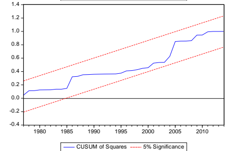
Fig. 3. CUSUM and CUSUMSQ tests on the ARDL models.
