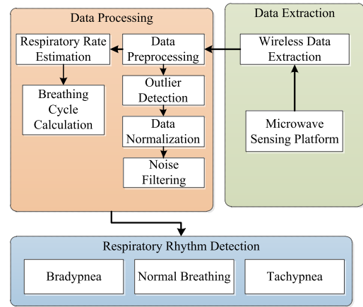
FIGURE 4. System architecture.
