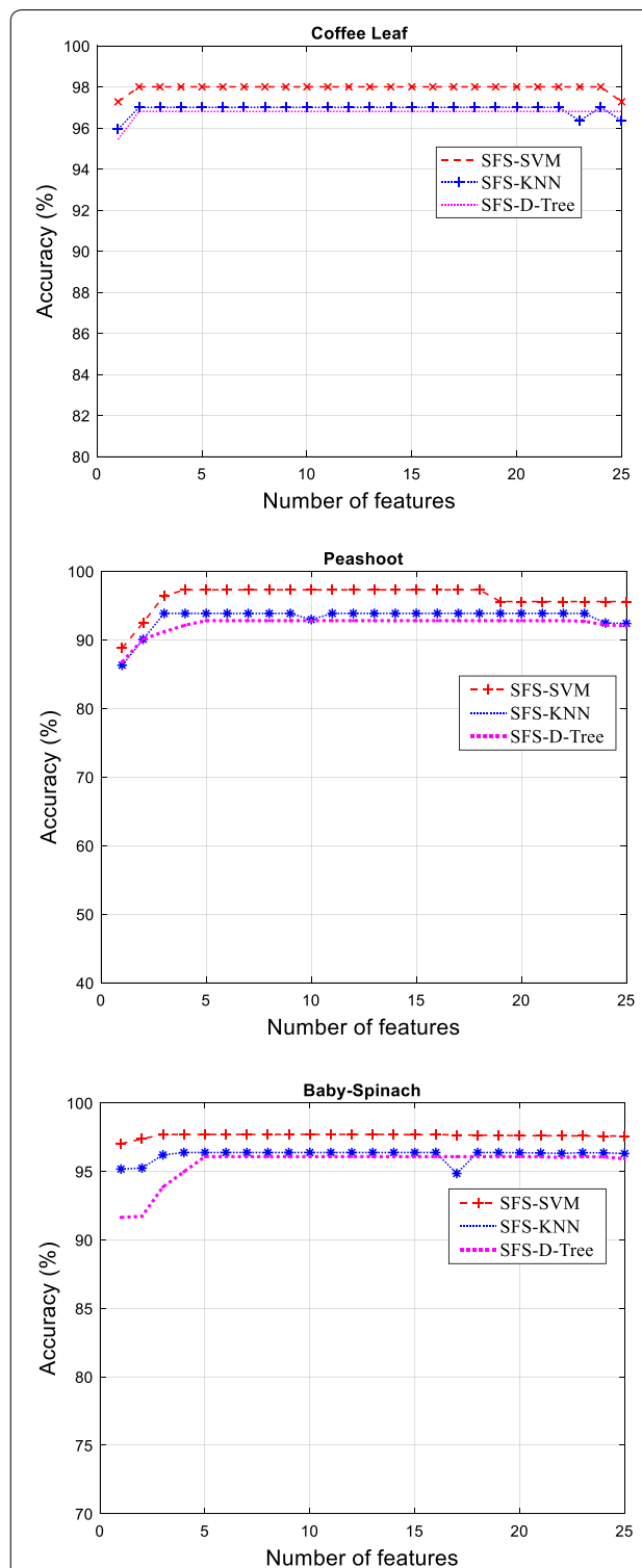
Fig. 6 Classification performance of classifiers using feature selection technique SFS for coffee, pea shoot and baby spinach leaves
