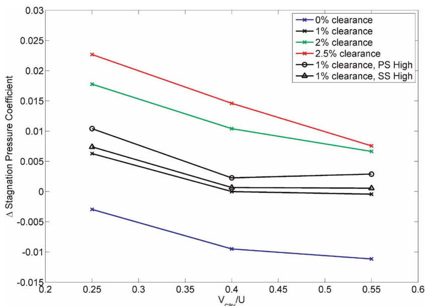
Figure 18. Overall change in the stagnation pressure coefficient as a result of misaligned hub platforms.
