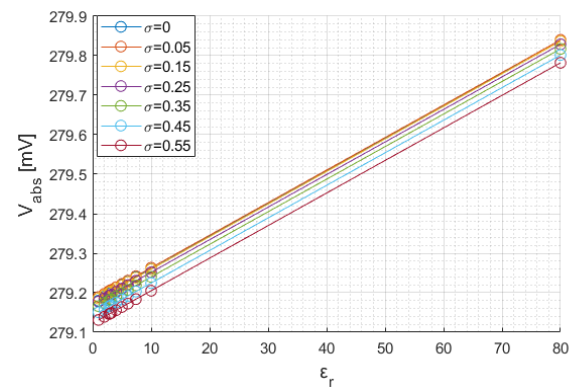
FIGURE 10. Change in amplitude of the induced voltage with relative permittivity changes for a given mixed flow conductivity range (0.05-0.55 S/m).
