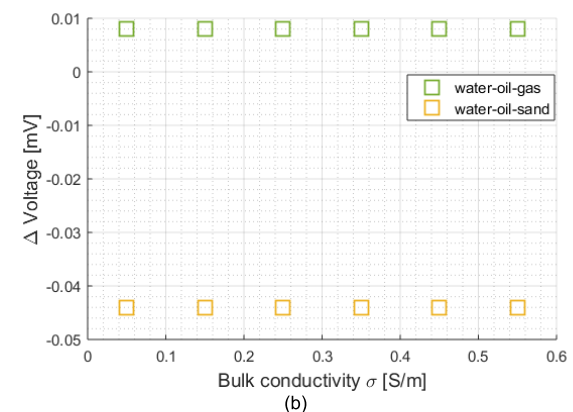
FIGURE 11. Induced voltage from (a) a trio of two-phase flows water-oil ( \epsilon_r = 2 ), water-gas ( \epsilon_r = 1 ), and water sand ( \epsilon_r = 7.4 ) and (b) the signal difference between the water-oil and the water-gas flows (labelled water-oil-gas) and the water-oil and the water-sand flows (labelled water-oil-sand) in low conductive environments ( \sigma = 0.05 -0.55 S/m).
