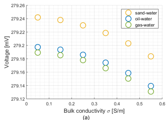
FIGURE 10. Change in amplitude of the induced voltage with relative permittivity changes for a given mixed flow conductivity range (0.05-0.55 S/m).
