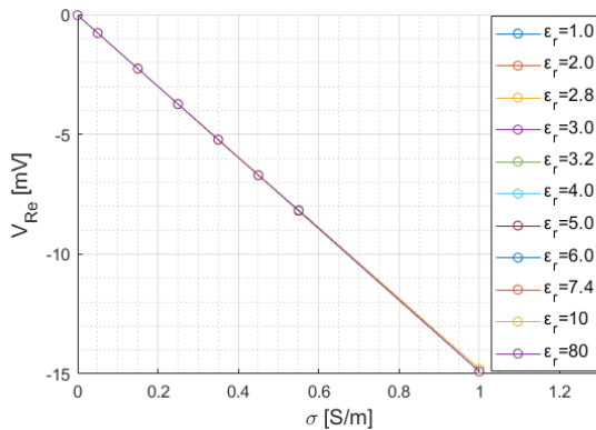
FIGURE 6. Effect of changes in conductivity on the real component of the measured amplitude.
