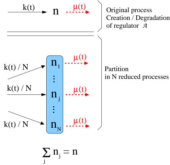
Figure 2. We partition each creation event into N 'types'. The creation rate associated to a particular type is given by k(t)/N . The sum of molecules numbers n_j over each type is equal to the total number of molecules n in the original model.
