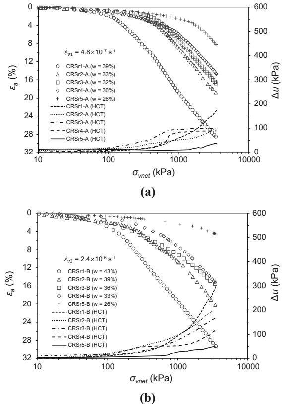
Fig. 13 CRS compression curves at different initial water contents: a \dot{\epsilon}_{v1} = 4.8 \times 10^{-7} \text{ s}^{-1} , b \dot{\epsilon}_{v2} = 2.4 \times 10^{-6} \text{ s}^{-1} (replotted from Bagheri et al. 2019)
