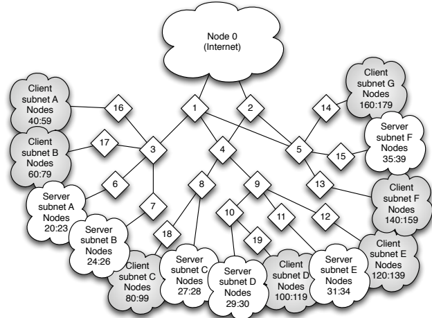
Figure 1. Simulated Network
