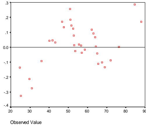
Fig. 2. Q-Q plot of students' average attention levels during the assessment exercise
