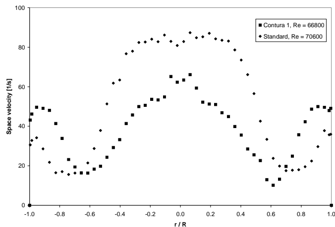
Figure 16. Experimental space velocity profiles for the Contura 1 and Standard substrate
