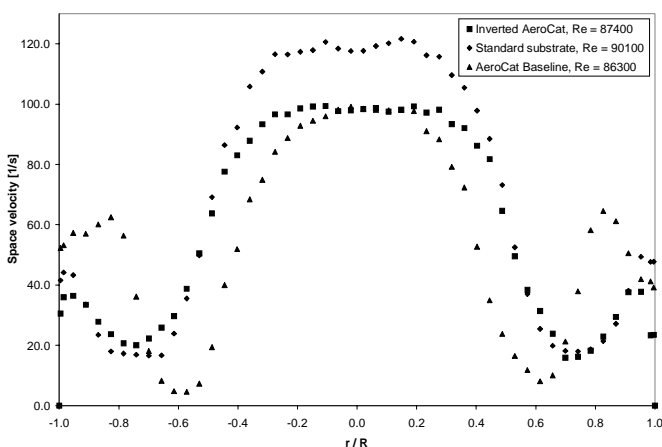
Figure 15. Comparison between the inverted AeroCat, AeroCat baseline and the Standard substrate
