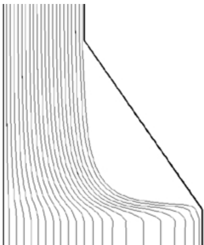
Figure 18. Particle tracks for the Standard substrate geometry
