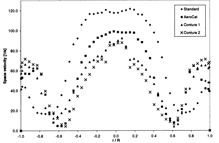
Figure 9. Flow distribution at Re = ~85000
