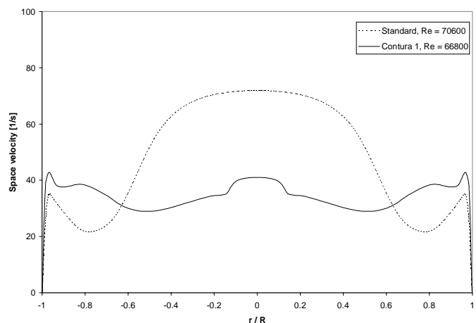
Figure 17. Predicted space velocity profiles for the Contura 1 and Standard substrate
