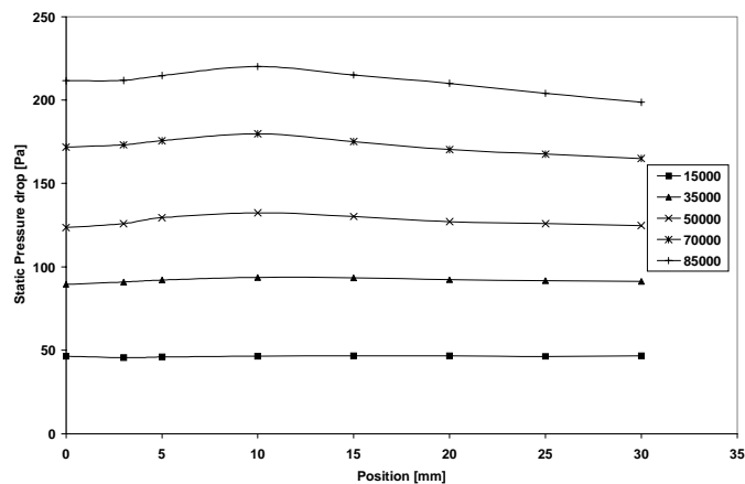
Figure 12. Contura 2 pressure drop at different positions and Re
