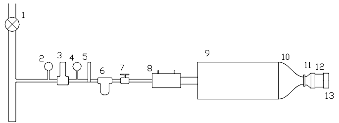
Figure 2. Schematic of iso-thermal flow rig
