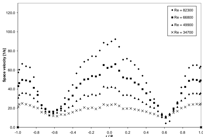
Figure 6. Flow distribution for Contura 1
