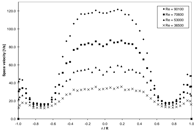
Figure 5. Flow distribution for the Standard substrate
