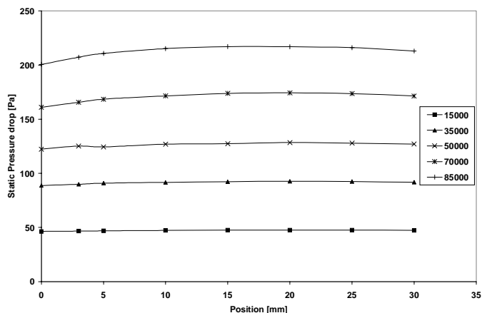
Figure 10. Standard substrate pressure drop at different positions and Re
