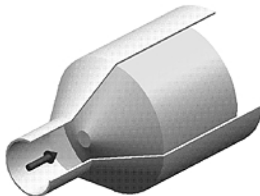
Figure 1. Contura substrate with diffuser
