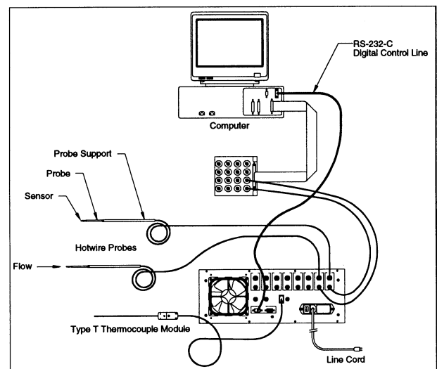
Figure 3. Overview of the IFA 300 System (Courtesy of TSI) [7]
