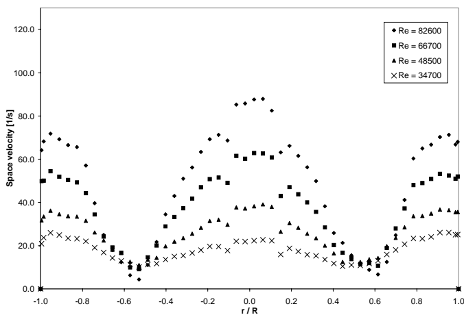
Figure 7. Flow distribution for Contura 2
