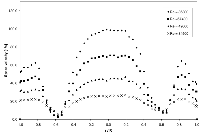
Figure 8. Flow distribution for AeroCat
