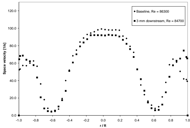
Figure 14. AeroCat in baseline position compared to the 3 mm downstream position
