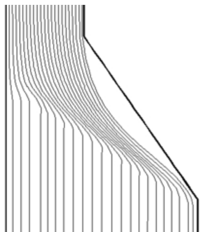
Figure 19. Particle tracks for the Contura 1 geometry
