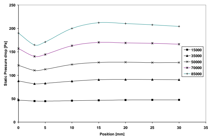
Figure 13. AeroCat pressure drop at different positions and Re
