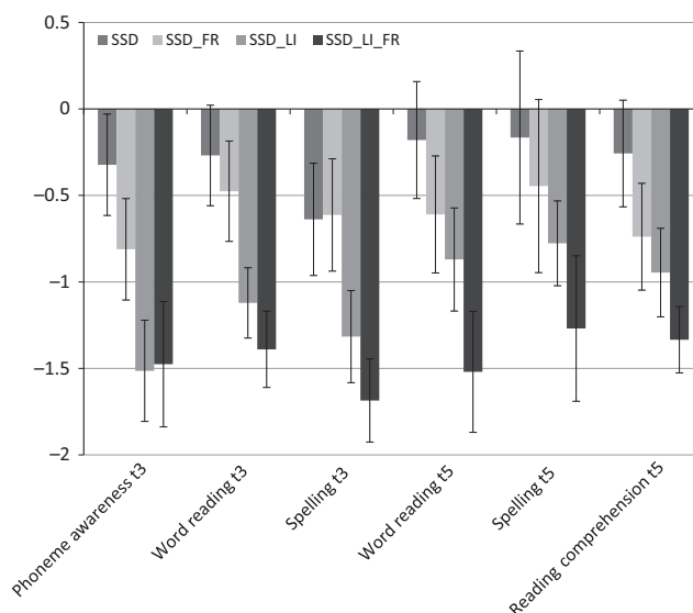
Figure 1 Mean scores for literacy outcome measures at age 8 for SSD according to subgroup. Scores are z-scores, referenced to the TD group mean, with 95% CIs
