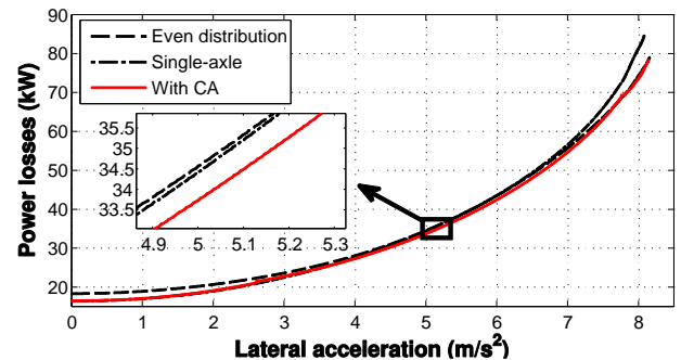
Fig. 9. Total drivetrain power losses (including tire power losses) simulated during the ramp steer maneuver for even distribution, single-axle, and the developed CA strategy
