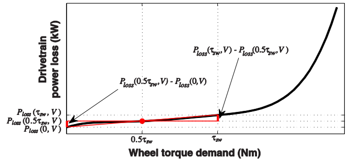
Fig. 2. Geometrical interpretation of Theorem 1, indicating the optimal switching point on the drivetrain power loss characteristic
