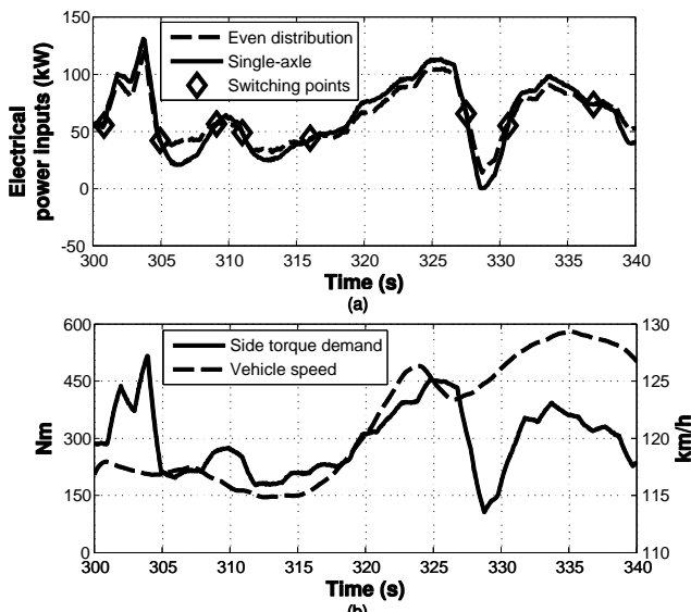
Fig. 7. Sample of driving cycle measurements: (a) electrical power input for the even distribution and single-axle strategies with the switching points indicated by markers; and (b) side torque demands overlapped with V
