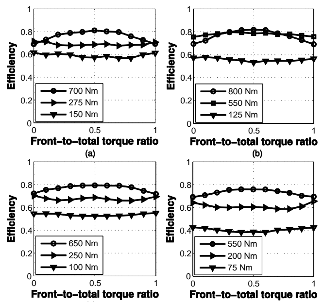
Fig. 5. Measured drivetrain efficiencies as a function of the front-to-total torque ratio, for different side torques at vehicle speeds of: (a) 40 km/h; (b) 65 km/h; (c) 90 km/h; and (d) 115 km/h
