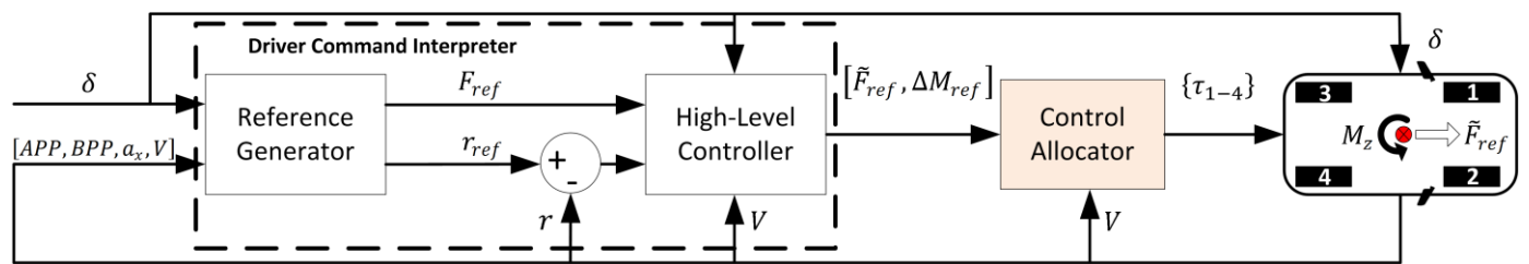
Fig. 1. The vehicle dynamics control structure
