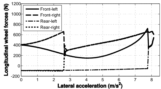
Fig. 8. Longitudinal wheel forces, simulated during the ramp steer maneuver at 100 km/h with the developed CA strategy. The outer and inner sides switch from single-axle to even distribution respectively at a_y of 2.6 and 7.8 m/s^2
