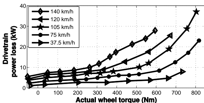
Fig. 4. The power losses of a single drivetrain, measured on the rolling road facility
