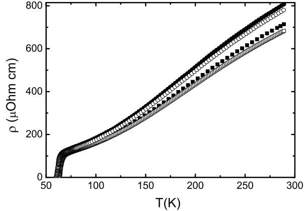
FIG. 1: In-plane resistivity of our HoBCO crystal as a function of T: dots - sample H21, P=0; squares - H22, P=0.48 GPa; open squares - H23, P=0.48 GPa after 5 days under pressure ; open circles - H24, P=0 after removing pressure.
