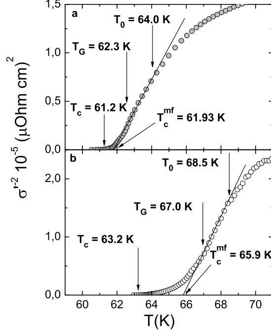
FIG. 3: \sigma'^{-2} as a function of T at P=0 (a) and P=0.48 GPa (b).
