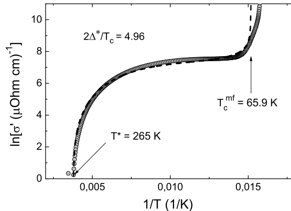
FIG. 6: \ln\sigma' vs 1/T (circles) compared with Eq. (10) (dashed line) plotted with \Delta^*(T_c)=156.7 K. P=0.48 GPa.
