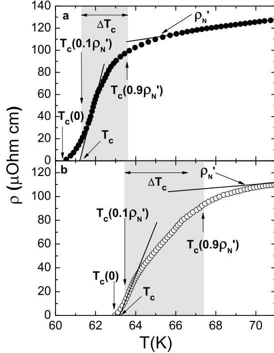
FIG. 2: Resistive transition of HoBCO single crystal at P=0 (a) and P=0.48 GPa (b).
