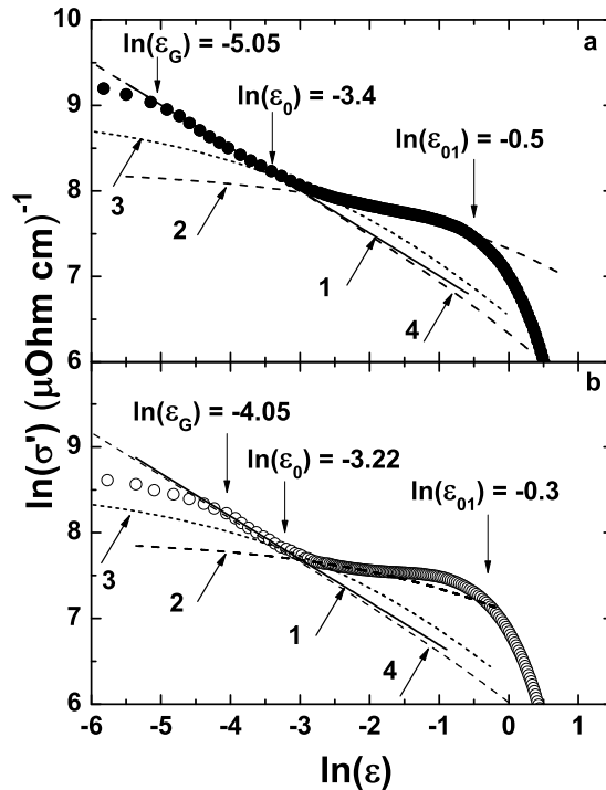
FIG. 4: \ln\sigma' vs \ln\varepsilon at P=0 (dots, a) and P=0.48 GPa (circles, b) compared with fluctuation theories: 1- 3D AL; 2 - MT with d = d_{01} ; 3 - MT with d = 11.67\text{\AA} ; 4 - LD.
