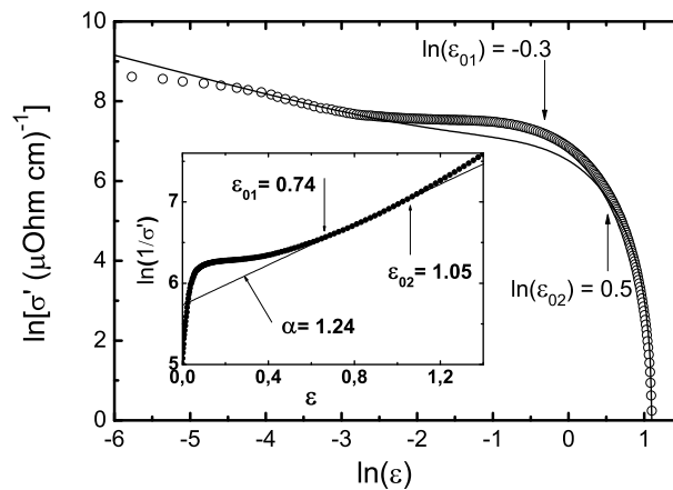
FIG. 5: \ln\sigma'(\ln\varepsilon) (circles) compared with Eq. (10) (solid line). Insert: \ln\sigma'^{-1} as a function of \varepsilon . P=0.48 GPa.
