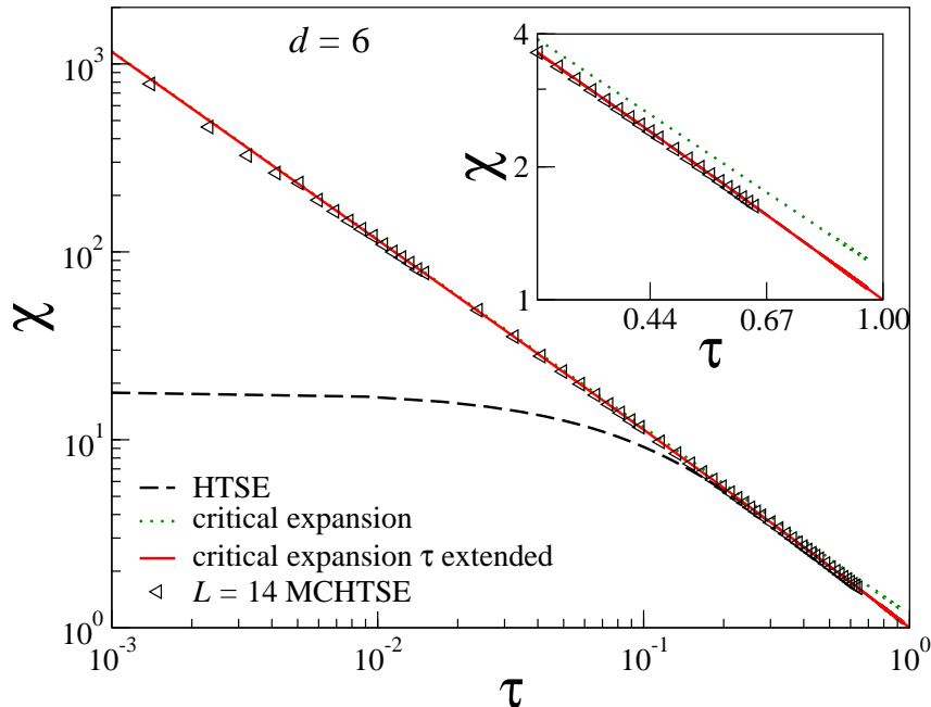
Figure 5: Extended scaling for the susceptibility of the Ising model in d = 6 dimensions. The extended scaling curve (solid, red online) traces the critical curve of [4] (dotted, green online) close to \tau = 0 and the HTSE [6] (dashed) close to \tau = 1 and as with the MCHTSE estimates in between.
